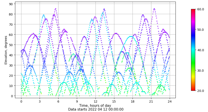
Time-elevation plot for station BCL1. Signal to Noise S1C Data file BCL100ESP_R_2022102.xtr
