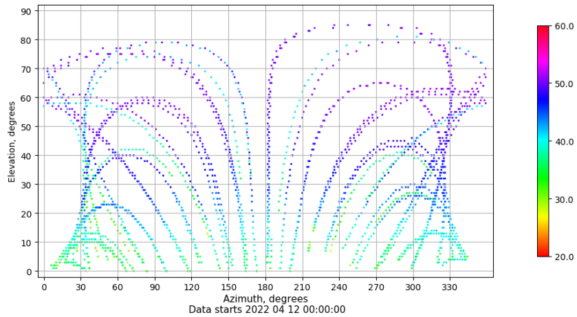
Azimuth-elevation plot for station BCL1. Signal to Noise S1C Data file BCL100ESP_R_2022102.xtr
