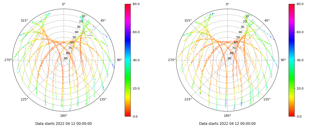
Skyplot for station BCL1. Parameter M1C Data file BCL100ESP_R_2022102.xtr Skyplot for station BCL1. Parameter M2P Data file BCL100ESP_R_2022102.xtr
