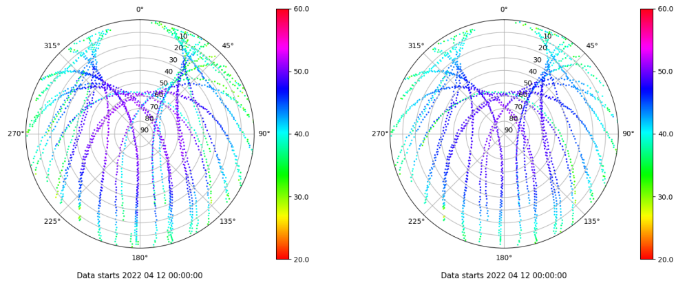
Skyplot for station BCL1. Signal to Noise S1C Data file BCL100ESP_R_2022102.xtr Skyplot for station BCL1. Signal to Noise S2P Data file BCL100ESP_R_2022102.xtr
