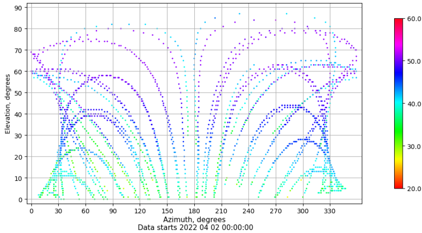
Azimuth-elevation plot for station BCL1. Signal to Noise S1C Data file BCL100ESP_R_2022092.xtr
