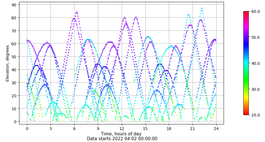
Time-elevation plot for station BCL1. Signal to Noise S1C Data file BCL100ESP_R_2022092.xtr
