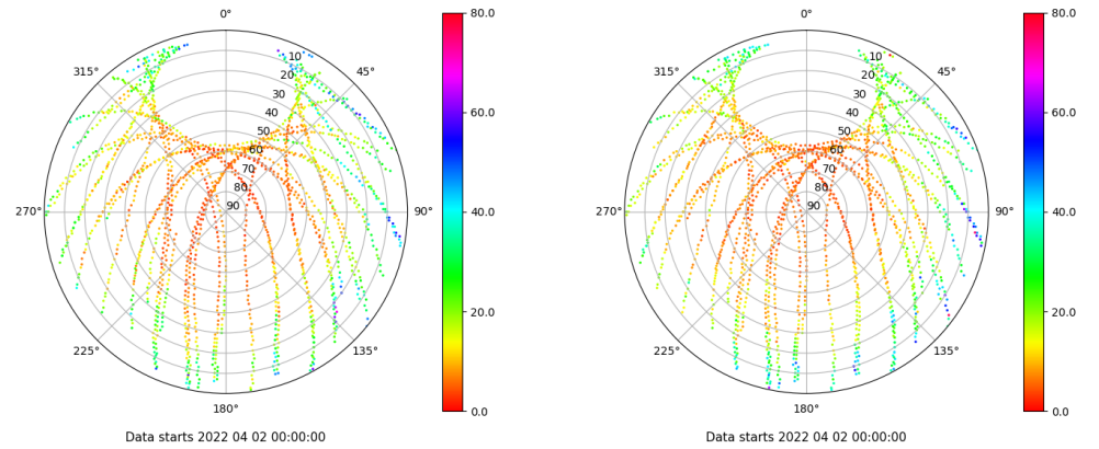
Skyplot for station BCL1. Parameter M1C Data file BCL100ESP_R_2022092.xtr Skyplot for station BCL1. Parameter M2P Data file BCL100ESP_R_2022092.xtr
