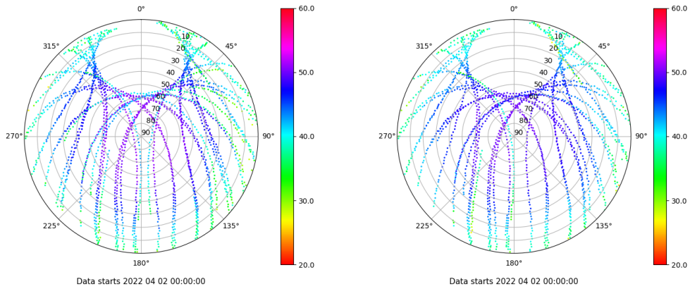
Skyplot for station BCL1. Signal to Noise S1C Data file BCL100ESP_R_2022092.xtr Skyplot for station BCL1. Signal to Noise S2P Data file BCL100ESP_R_2022092.xtr
