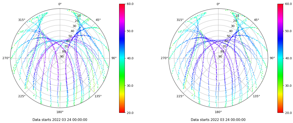
Skyplot for station BCL1. Signal to Noise S1C Data file BCL100ESP_R_2022083.xtr Skyplot for station BCL1. Signal to Noise S2P Data file BCL100ESP_R_2022083.xtr
