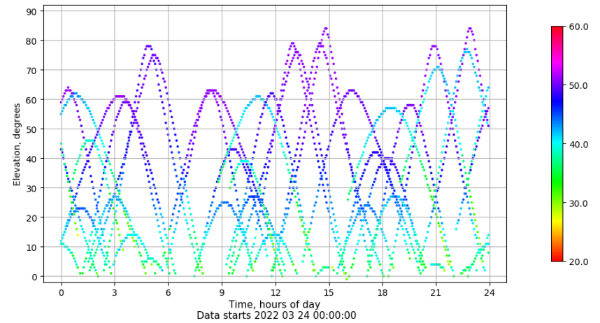
Time-elevation plot for station BCL1. Signal to Noise S1C Data file BCL100ESP_R_2022083.xtr
