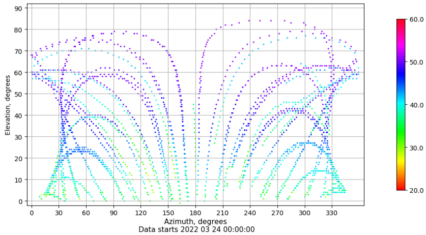
Azimuth-elevation plot for station BCL1. Signal to Noise S1C Data file BCL100ESP_R_2022083.xtr
