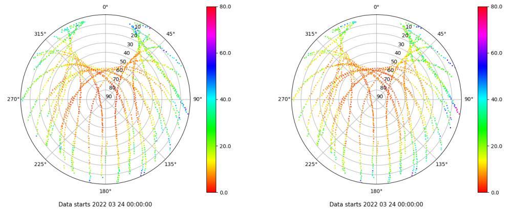
Skyplot for station BCL1. Parameter M1C Data file BCL100ESP_R_2022083.xtr Skyplot for station BCL1. Parameter M2P Data file BCL100ESP_R_2022083.xtr
