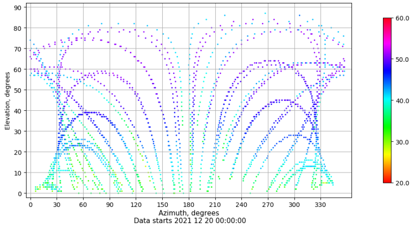
Azimuth-elevation plot for station BCL1. Signal to Noise S1C Data file BCL100ESP_R_2021354.xtr
