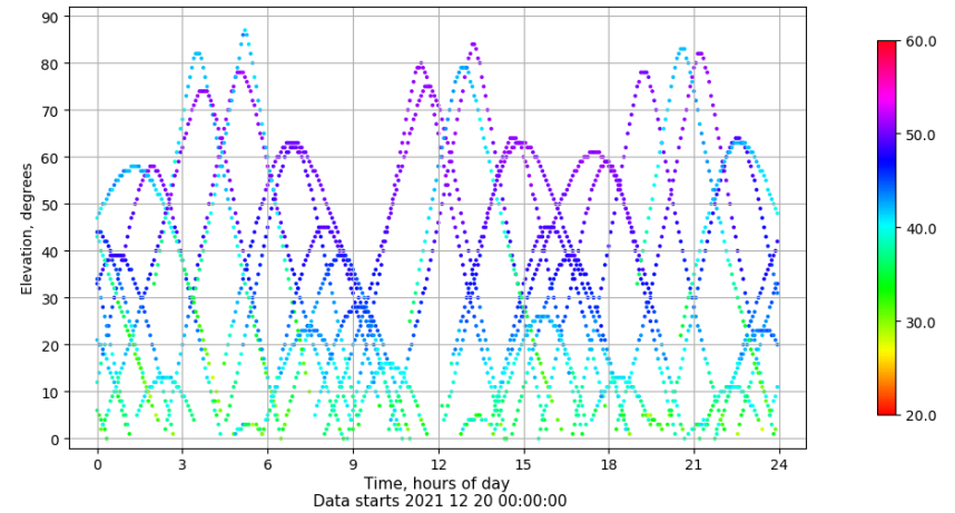
Time-elevation plot for station BCL1. Signal to Noise S1C Data file BCL100ESP_R_2021354.xtr
