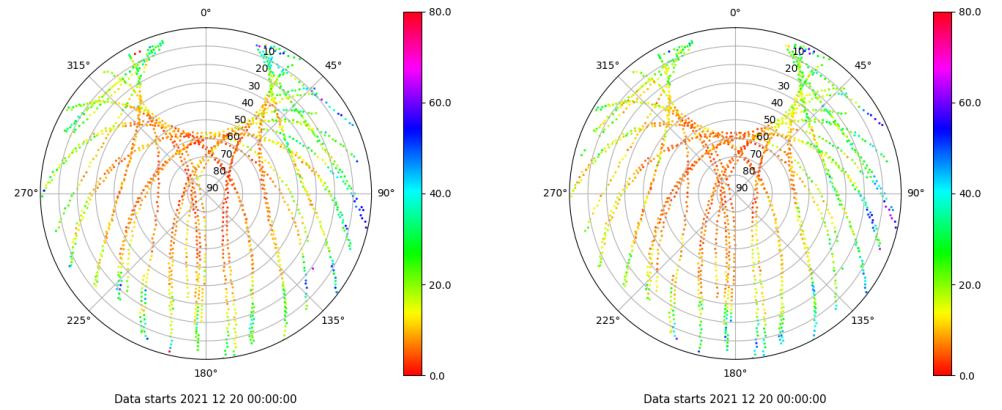
Skyplot for station BCL1. Parameter M1C Data file BCL100ESP_R_2021354.xtr Skyplot for station BCL1. Parameter M2P Data file BCL100ESP_R_2021354.xtr
