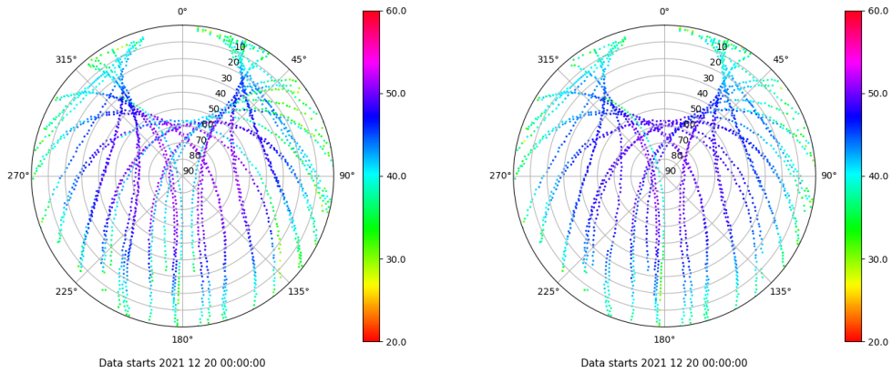
Skyplot for station BCL1. Signal to Noise S1C Data file BCL100ESP_R_2021354.xtr Skyplot for station BCL1. Signal to Noise S2P Data file BCL100ESP_R_2021354.xtr
