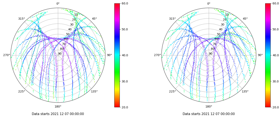
Skyplot for station BCL1. Signal to Noise S1C Data file BCL100ESP_R_2021341.xtr Skyplot for station BCL1. Signal to Noise S2P Data file BCL100ESP_R_2021341.xtr
