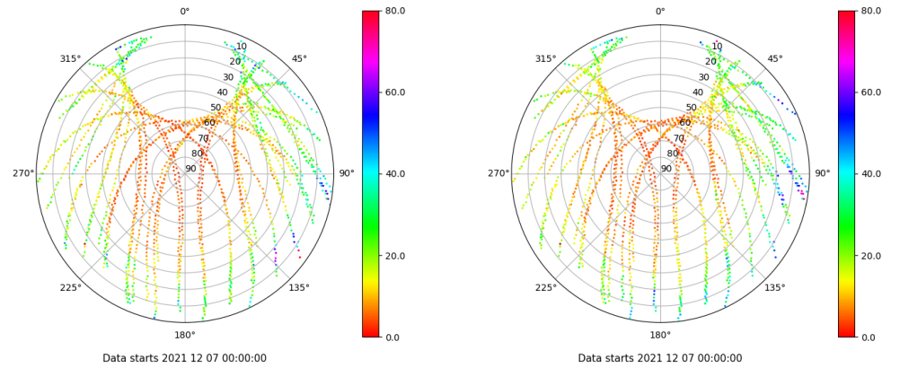
Skyplot for station BCL1. Parameter M1C Data file BCL100ESP_R_2021341.xtr Skyplot for station BCL1. Parameter M2P Data file BCL100ESP_R_2021341.xtr
