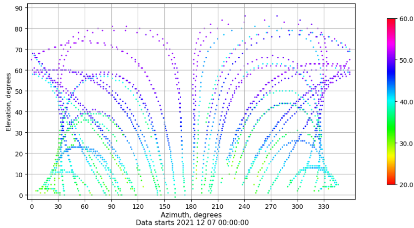
Azimuth-elevation plot for station BCL1. Signal to Noise S1C Data file BCL100ESP_R_2021341.xtr
