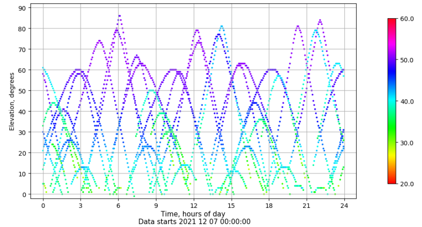
Time-elevation plot for station BCL1. Signal to Noise S1C Data file BCL100ESP_R_2021341.xtr
