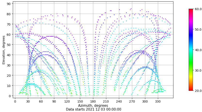
Azimuth-elevation plot for station BCL1. Signal to Noise S1C Data file BCL100ESP_R_2021337.xtr
