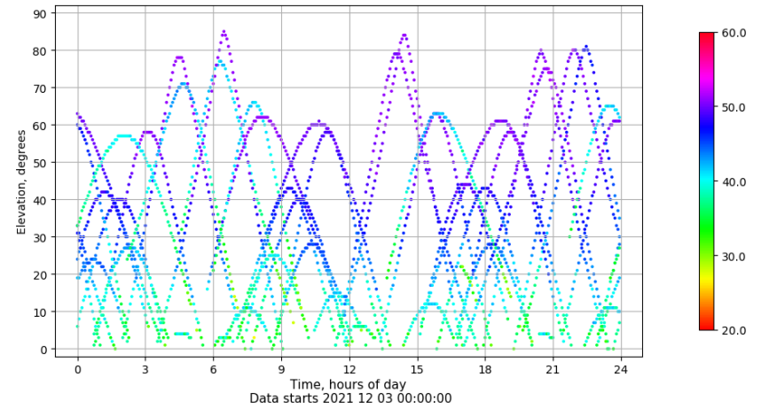
Time-elevation plot for station BCL1. Signal to Noise S1C Data file BCL100ESP_R_2021337.xtr
