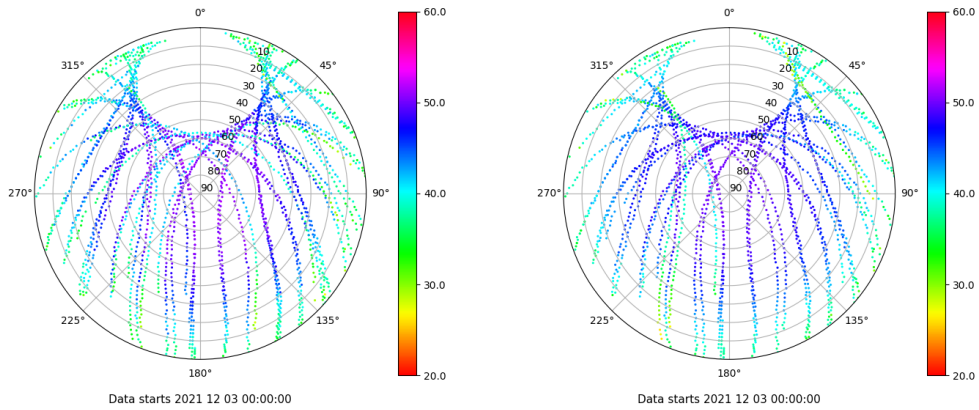
Skyplot for station BCL1. Signal to Noise S1C Data file BCL100ESP_R_2021337.xtr Skyplot for station BCL1. Signal to Noise S2P Data file BCL100ESP_R_2021337.xtr
