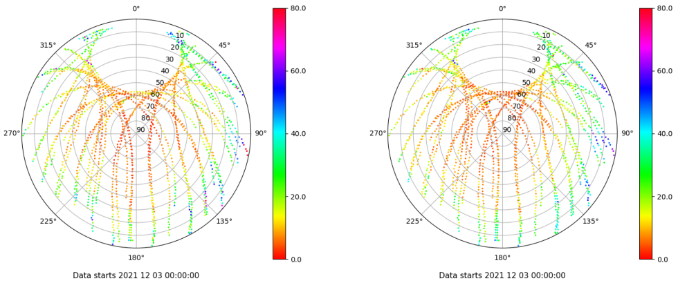
Skyplot for station BCL1. Parameter M1C Data file BCL100ESP_R_2021337.xtr Skyplot for station BCL1. Parameter M2P Data file BCL100ESP_R_2021337.xtr
