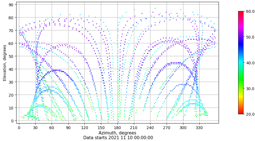
Azimuth-elevation plot for station BCL1. Signal to Noise S1C Data file BCL100ESP_R_2021314.xtr
