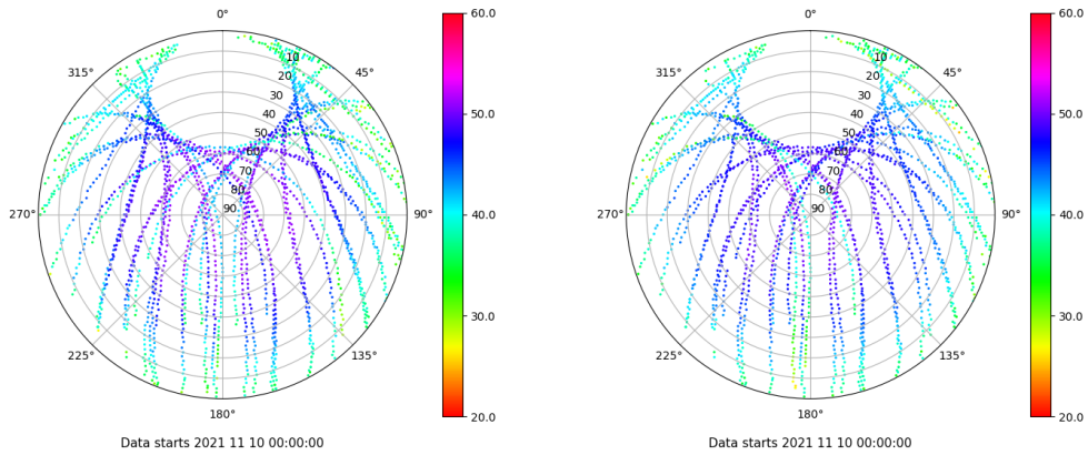
Skyplot for station BCL1. Signal to Noise S1C Data file BCL100ESP_R_2021314.xtr Skyplot for station BCL1. Signal to Noise S2P Data file BCL100ESP_R_2021314.xtr
