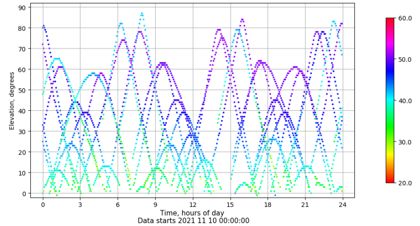
Time-elevation plot for station BCL1. Signal to Noise S1C Data file BCL100ESP_R_2021314.xtr
