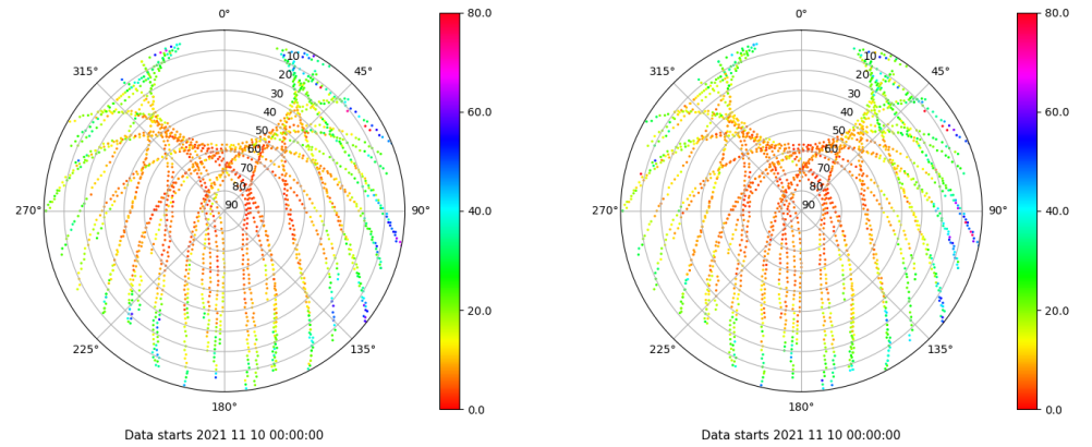
Skyplot for station BCL1. Parameter M1C Data file BCL100ESP_R_2021314.xtr Skyplot for station BCL1. Parameter M2P Data file BCL100ESP_R_2021314.xtr
