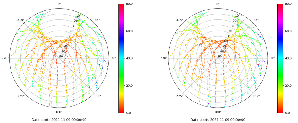
Skyplot for station BCL1. Parameter M1C Data file BCL100ESP_R_2021313.xtr Skyplot for station BCL1. Parameter M2P Data file BCL100ESP_R_2021313.xtr
