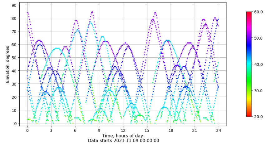
Time-elevation plot for station BCL1. Signal to Noise S1C Data file BCL100ESP_R_2021313.xtr
