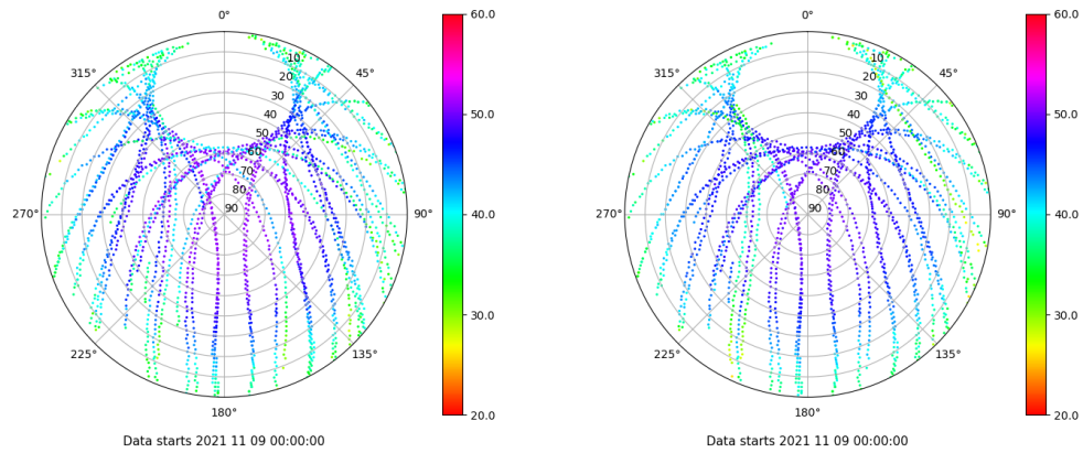
Skyplot for station BCL1. Signal to Noise S1C Data file BCL100ESP_R_2021313.xtr Skyplot for station BCL1. Signal to Noise S2P Data file BCL100ESP_R_2021313.xtr
