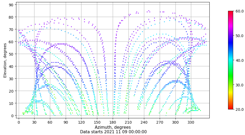
Azimuth-elevation plot for station BCL1. Signal to Noise S1C Data file BCL100ESP_R_2021313.xtr
