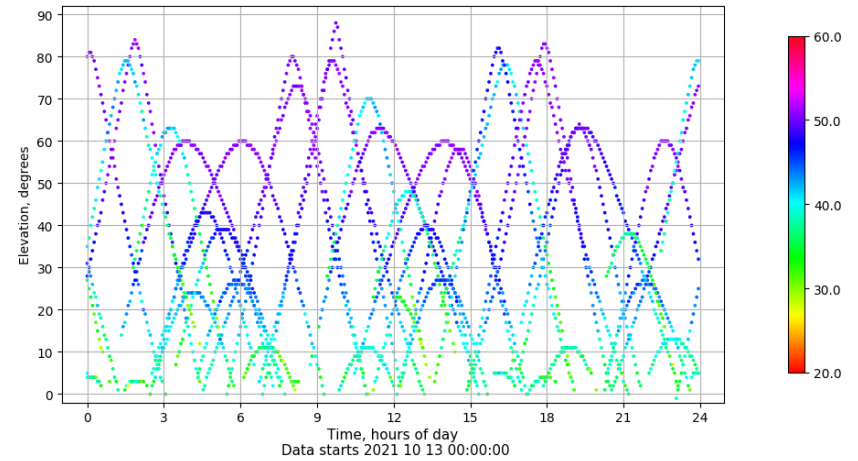
Time-elevation plot for station BCL1. Signal to Noise S1C Data file BCL100ESP_R_2021286.xtr
