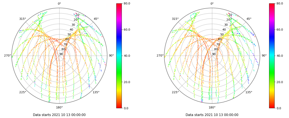
Skyplot for station BCL1. Parameter M1C Data file BCL100ESP_R_2021286.xtr Skyplot for station BCL1. Parameter M2P Data file BCL100ESP_R_2021286.xtr
