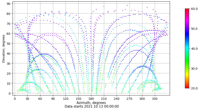
Azimuth-elevation plot for station BCL1. Signal to Noise S1C Data file BCL100ESP_R_2021286.xtr
