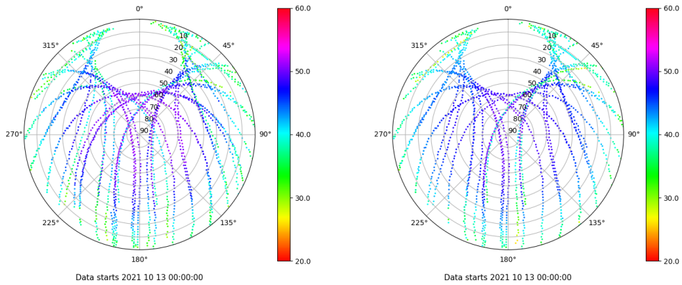
Skyplot for station BCL1. Signal to Noise S1C Data file BCL100ESP_R_2021286.xtr Skyplot for station BCL1. Signal to Noise S2P Data file BCL100ESP_R_2021286.xtr
