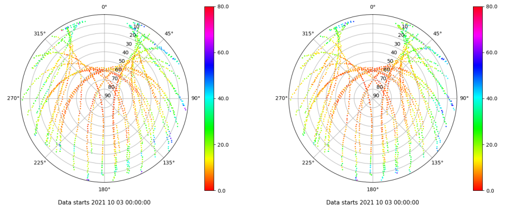
Skyplot for station BCL1. Parameter M1C Data file BCL100ESP_R_2021276.xtr Skyplot for station BCL1. Parameter M2P Data file BCL100ESP_R_2021276.xtr
