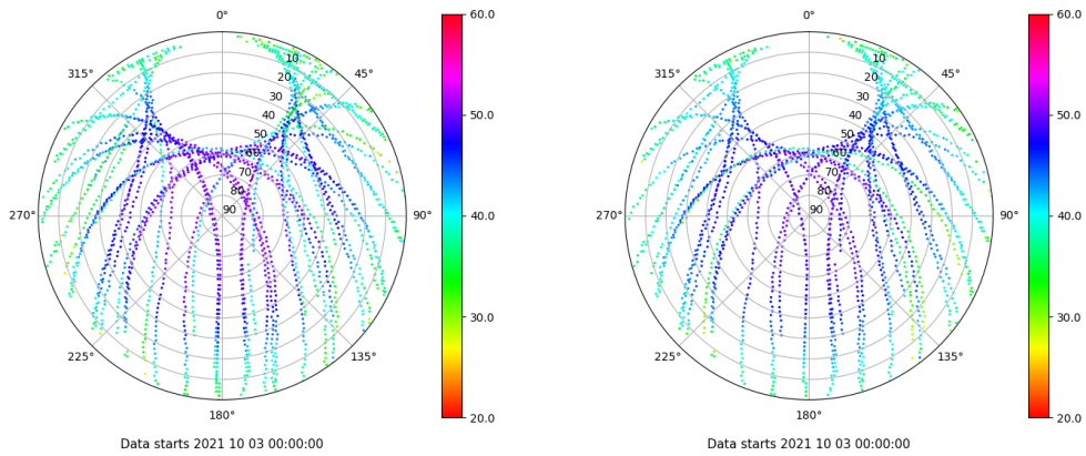
Skyplot for station BCL1. Signal to Noise S1C Data file BCL100ESP_R_2021276.xtr Skyplot for station BCL1. Signal to Noise S2P Data file BCL100ESP_R_2021276.xtr
