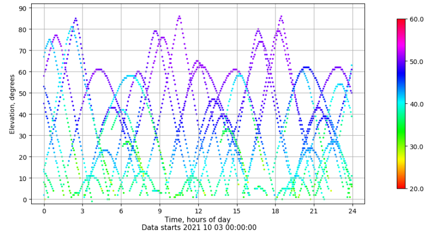
Time-elevation plot for station BCL1. Signal to Noise S1C Data file BCL100ESP_R_2021276.xtr
