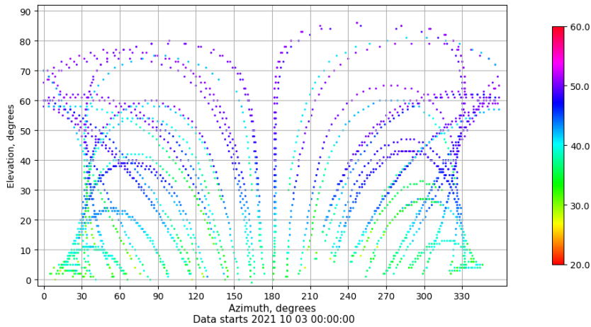
Azimuth-elevation plot for station BCL1. Signal to Noise S1C Data file BCL100ESP_R_2021276.xtr
