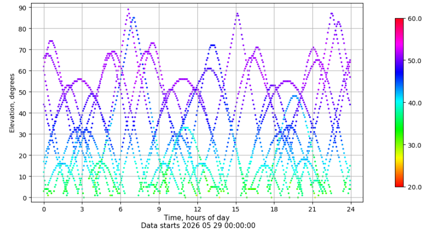
Time-elevation plot for station BADI. Signal to Noise S1C Data file BADI00ESP_R_2026149.xtr
