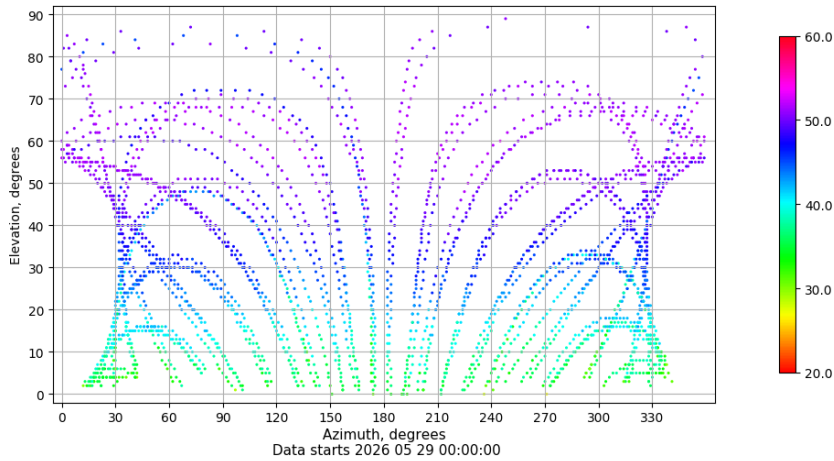
Azimuth-elevation plot for station BADI. Signal to Noise S1C Data file BADI00ESP_R_2026149.xtr
