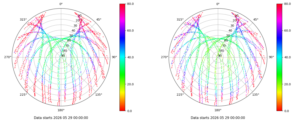
Skyplot for station BADI. Parameter M1C Data file BADI00ESP_R_2026149.xtr Skyplot for station BADI. Parameter M2C Data file BADI00ESP_R_2026149.xtr
