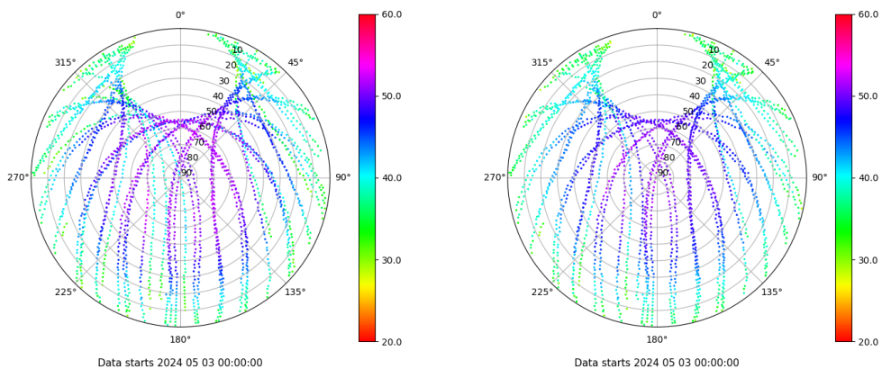
Skyplot for station BADI. Signal to Noise S1C Data file BADI00ESP_R_2024124.xtr Skyplot for station BADI. Signal to Noise S2C Data file BADI00ESP_R_2024124.xtr
