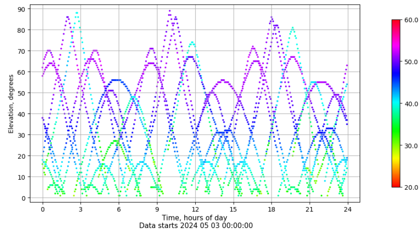
Time-elevation plot for station BADI. Signal to Noise S1C Data file BADI00ESP_R_2024124.xtr
