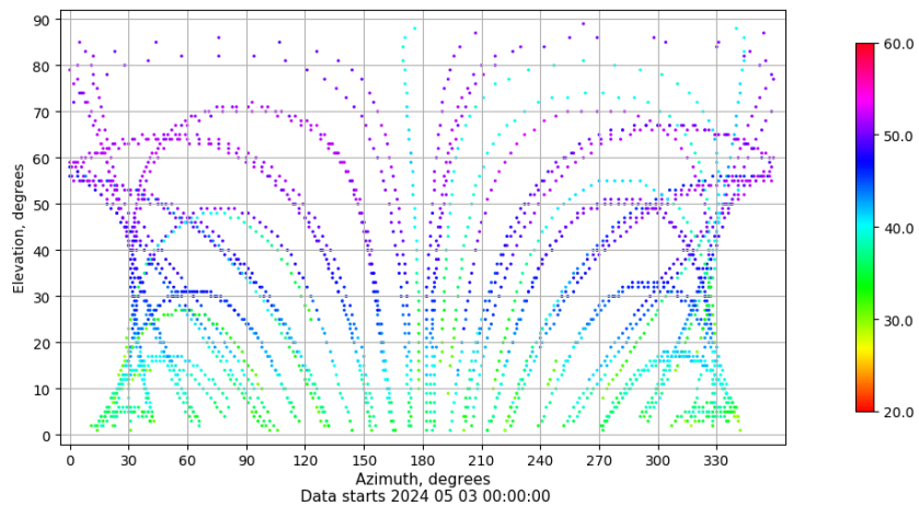
Azimuth-elevation plot for station BADI. Signal to Noise S1C Data file BADI00ESP_R_2024124.xtr
