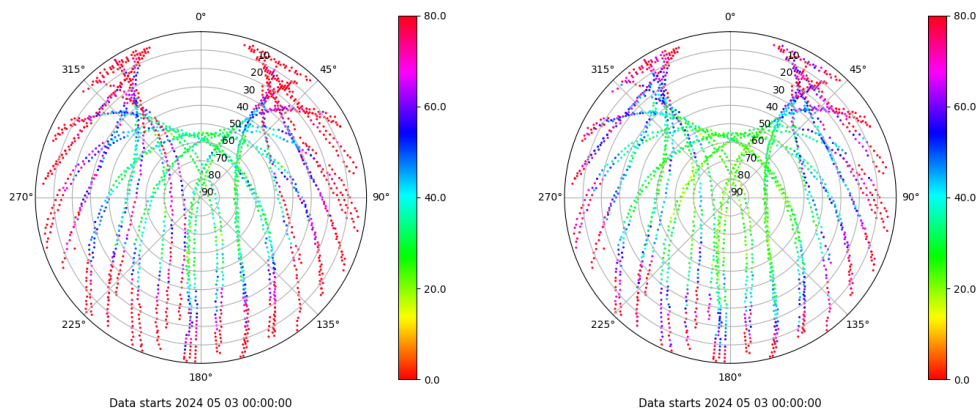
Skyplot for station BADI. Parameter M1C Data file BADI00ESP_R_2024124.xtr Skyplot for station BADI. Parameter M2C Data file BADI00ESP_R_2024124.xtr
