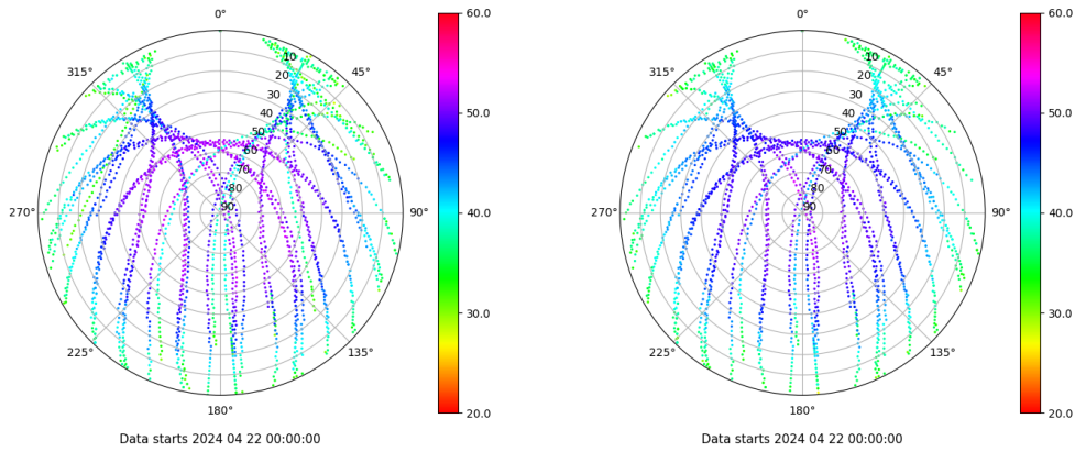
Skyplot for station BADI. Signal to Noise S1C Data file BADI00ESP_R_2024113.xtr Skyplot for station BADI. Signal to Noise S2C Data file BADI00ESP_R_2024113.xtr
