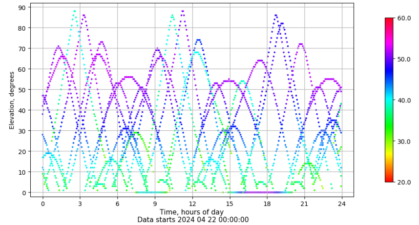
Time-elevation plot for station BADI. Signal to Noise S1C Data file BADI00ESP_R_2024113.xtr
