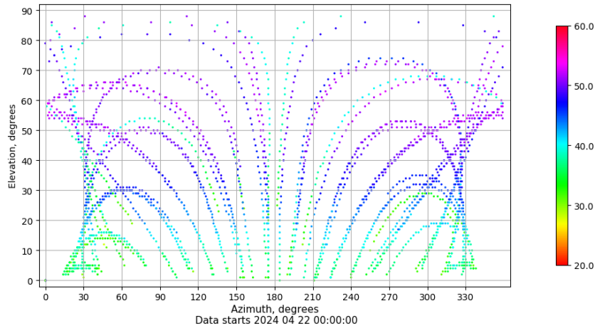
Azimuth-elevation plot for station BADI. Signal to Noise S1C Data file BADI00ESP_R_2024113.xtr
