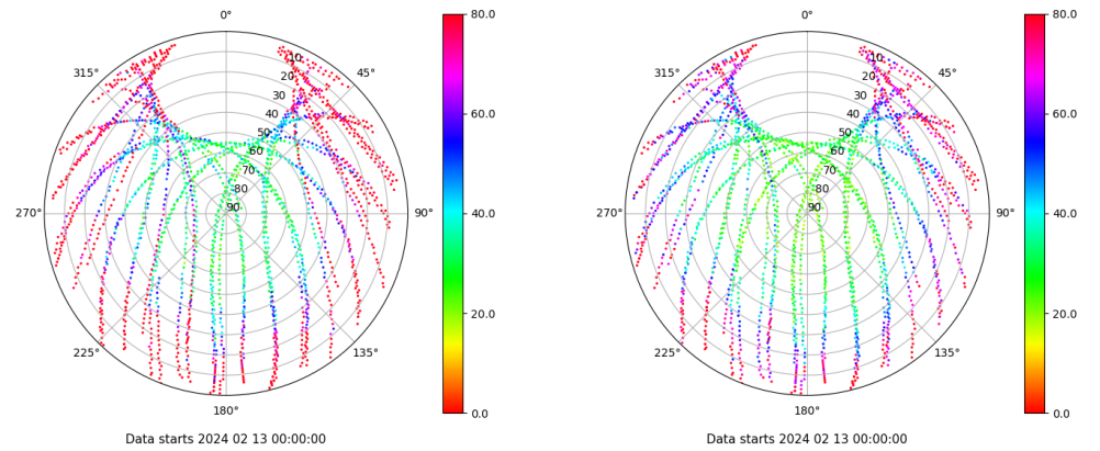
Skyplot for station BADI. Parameter M1C Data file BADI00ESP_R_2024044.xtr Skyplot for station BADI. Parameter M2C Data file BADI00ESP_R_2024044.xtr
