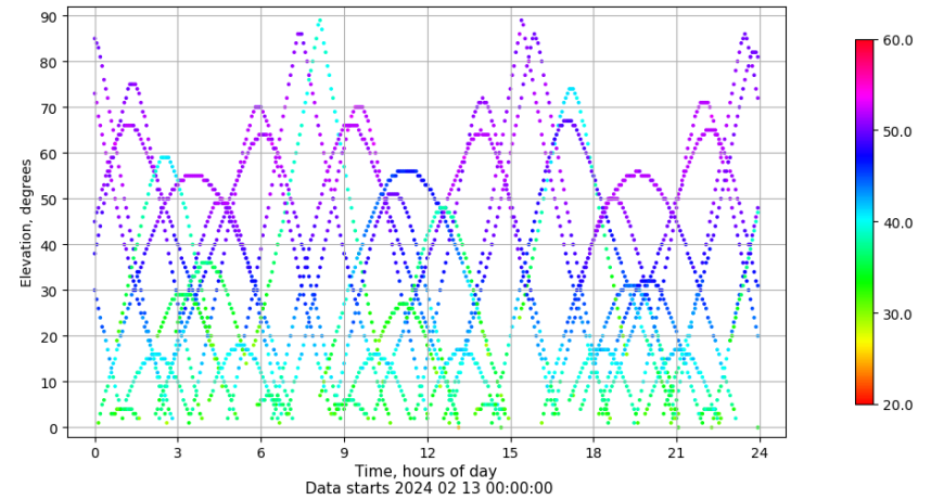
Time-elevation plot for station BADI. Signal to Noise S1C Data file BADI00ESP_R_2024044.xtr
