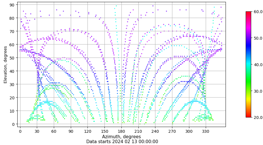
Azimuth-elevation plot for station BADI. Signal to Noise S1C Data file BADI00ESP_R_2024044.xtr
