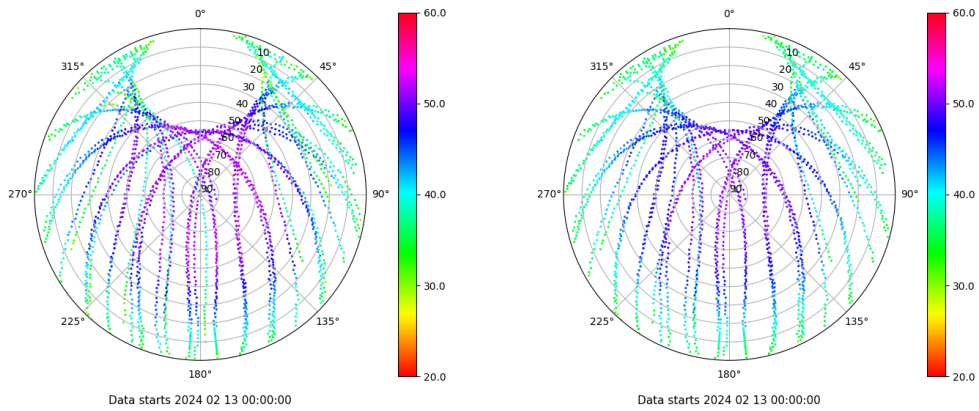
Skyplot for station BADI. Signal to Noise S1C Data file BADI00ESP_R_2024044.xtr Skyplot for station BADI. Signal to Noise S2C Data file BADI00ESP_R_2024044.xtr
