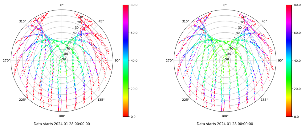
Skyplot for station BADI. Parameter M1C Data file BADI00ESP_R_2024028.xtr Skyplot for station BADI. Parameter M2C Data file BADI00ESP_R_2024028.xtr
