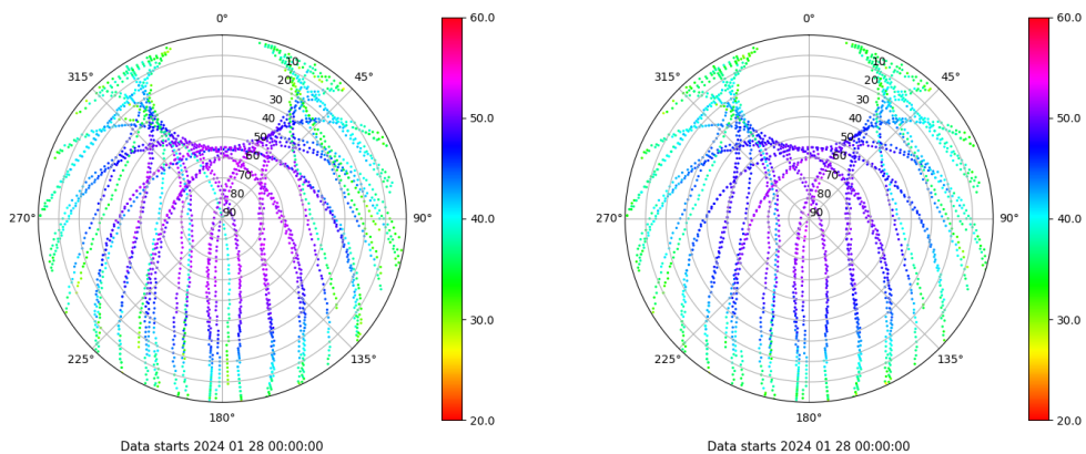
Skyplot for station BADI. Signal to Noise S1C Data file BADI00ESP_R_2024028.xtr Skyplot for station BADI. Signal to Noise S2C Data file BADI00ESP_R_2024028.xtr
