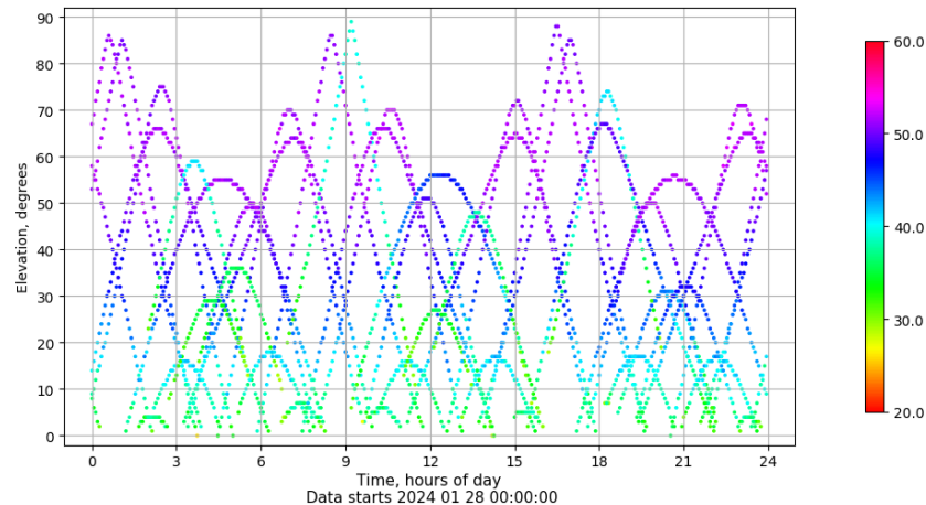
Time-elevation plot for station BADI. Signal to Noise S1C Data file BADI00ESP_R_2024028.xtr
