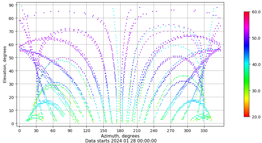
Azimuth-elevation plot for station BADI. Signal to Noise S1C Data file BADI00ESP_R_2024028.xtr
