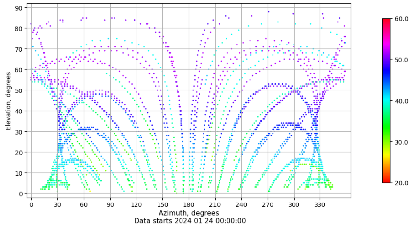
Azimuth-elevation plot for station BADI. Signal to Noise S1C Data file BADI00ESP_R_2024024.xtr
