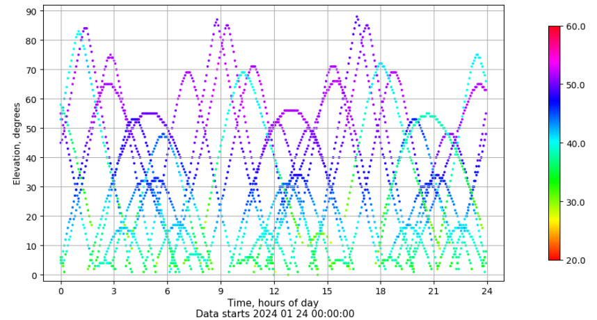
Time-elevation plot for station BADI. Signal to Noise S1C Data file BADI00ESP_R_2024024.xtr
