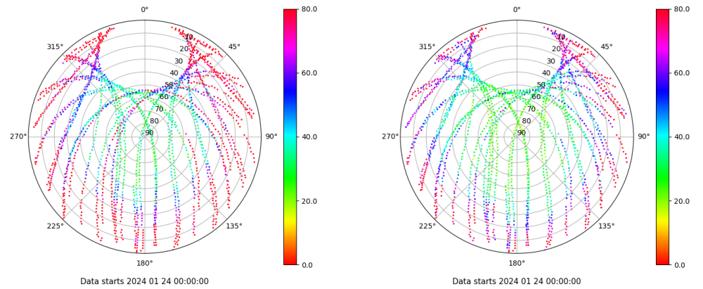
Skyplot for station BADI. Parameter M1C Data file BADI00ESP_R_2024024.xtr Skyplot for station BADI. Parameter M2C Data file BADI00ESP_R_2024024.xtr
