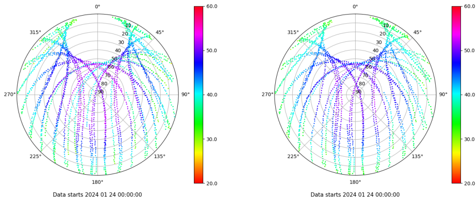
Skyplot for station BADI. Signal to Noise S1C Data file BADI00ESP_R_2024024.xtr Skyplot for station BADI. Signal to Noise S2C Data file BADI00ESP_R_2024024.xtr
