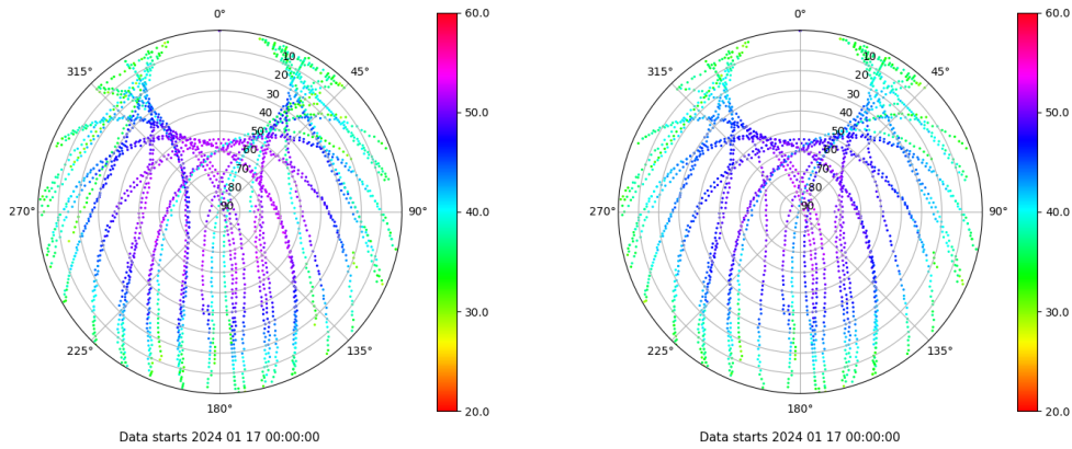
Skyplot for station BADI. Signal to Noise S1C Data file BADI00ESP_R_2024017.xtr Skyplot for station BADI. Signal to Noise S2C Data file BADI00ESP_R_2024017.xtr
