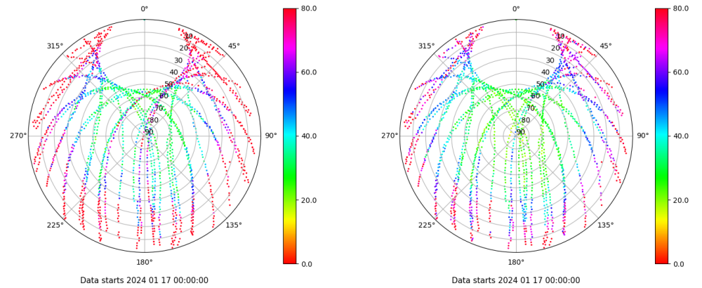
Skyplot for station BADI. Parameter M1C Data file BADI00ESP_R_2024017.xtr Skyplot for station BADI. Parameter M2C Data file BADI00ESP_R_2024017.xtr
