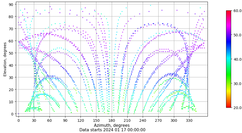
Azimuth-elevation plot for station BADI. Signal to Noise S1C Data file BADI00ESP_R_2024017.xtr
