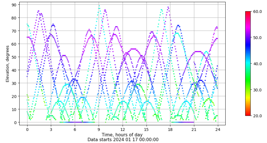
Time-elevation plot for station BADI. Signal to Noise S1C Data file BADI00ESP_R_2024017.xtr
