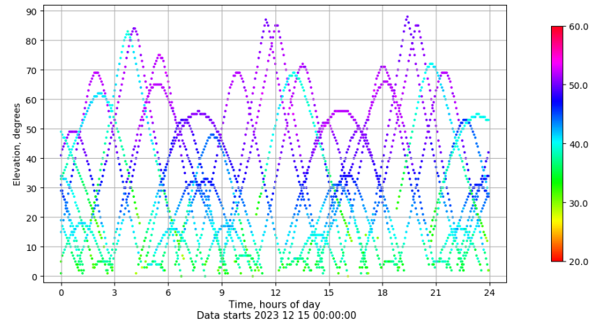
Time-elevation plot for station BADI. Signal to Noise S1C Data file BADI00ESP_R_2023349.xtr
