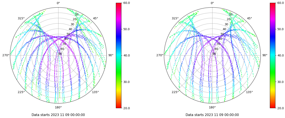
Skyplot for station BADI. Signal to Noise S1C Data file BADI00ESP_R_2023313.xtr Skyplot for station BADI. Signal to Noise S2C Data file BADI00ESP_R_2023313.xtr
