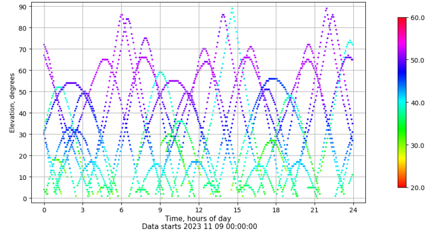
Time-elevation plot for station BADI. Signal to Noise S1C Data file BADI00ESP_R_2023313.xtr
