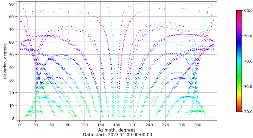
Azimuth-elevation plot for station BADI. Signal to Noise S1C Data file BADI00ESP_R_2023313.xtr
