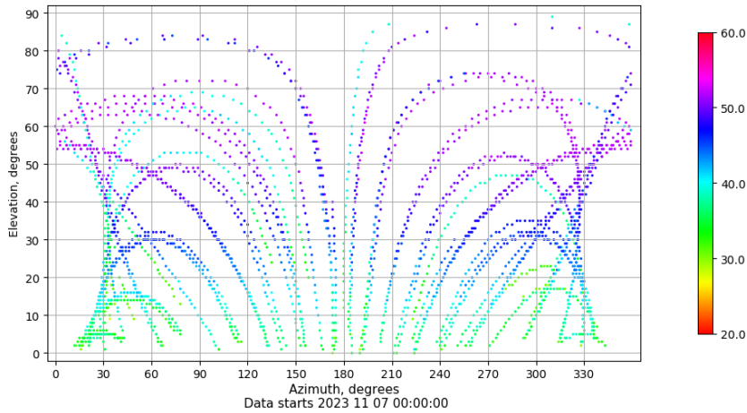
Azimuth-elevation plot for station BADI. Signal to Noise S1C Data file BADI00ESP_R_2023311.xtr
