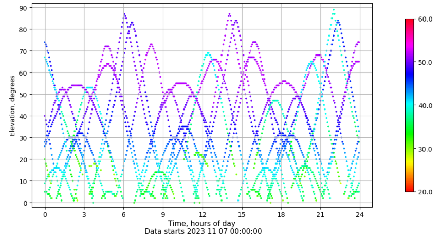
Time-elevation plot for station BADI. Signal to Noise S1C Data file BADI00ESP_R_2023311.xtr
