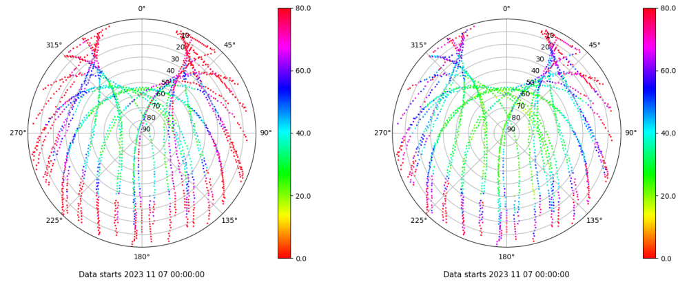
Skyplot for station BADI. Parameter M1C Data file BADI00ESP_R_2023311.xtr Skyplot for station BADI. Parameter M2C Data file BADI00ESP_R_2023311.xtr
