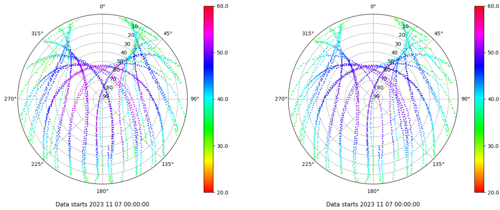
Skyplot for station BADI. Signal to Noise S1C Data file BADI00ESP_R_2023311.xtr Skyplot for station BADI. Signal to Noise S2C Data file BADI00ESP_R_2023311.xtr
