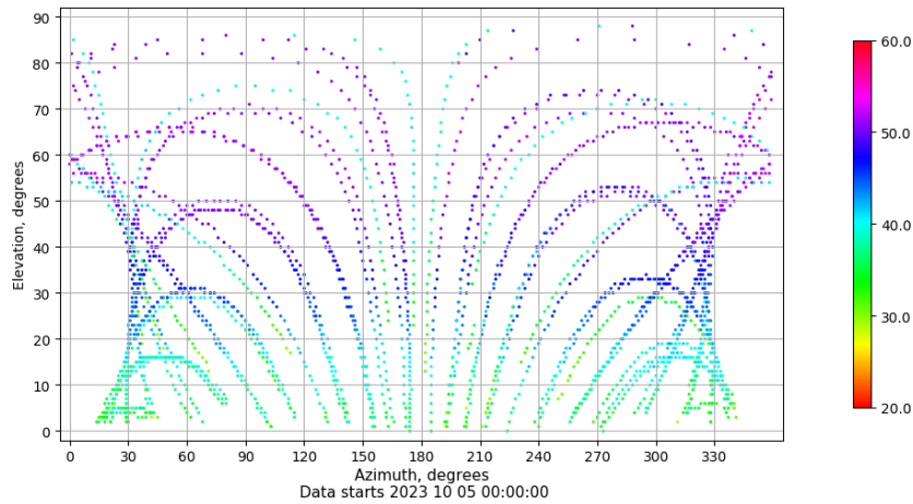
Azimuth-elevation plot for station BADI. Signal to Noise S1C Data file BADI00ESP_R_2023278.xtr
