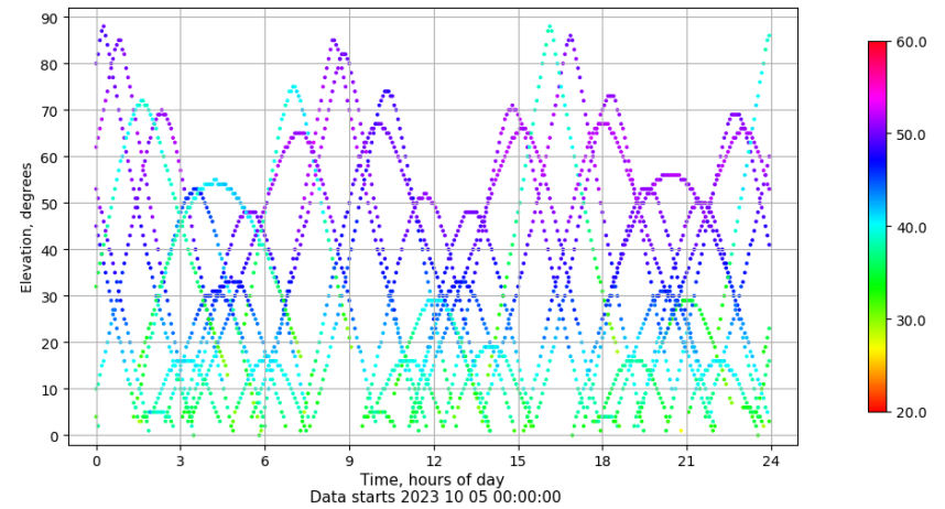
Time-elevation plot for station BADI. Signal to Noise S1C Data file BADI00ESP_R_2023278.xtr
