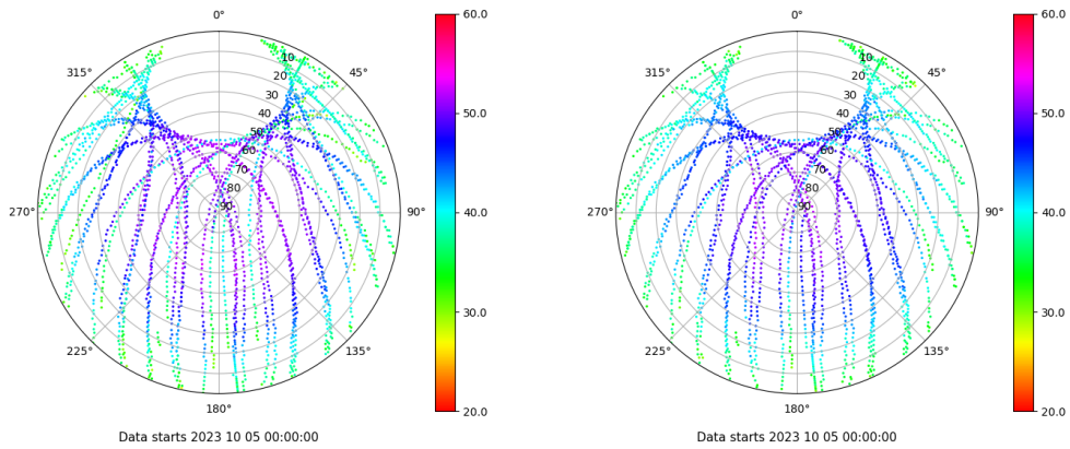
Skyplot for station BADI. Signal to Noise S1C Data file BADI00ESP_R_2023278.xtr Skyplot for station BADI. Signal to Noise S2C Data file BADI00ESP_R_2023278.xtr
