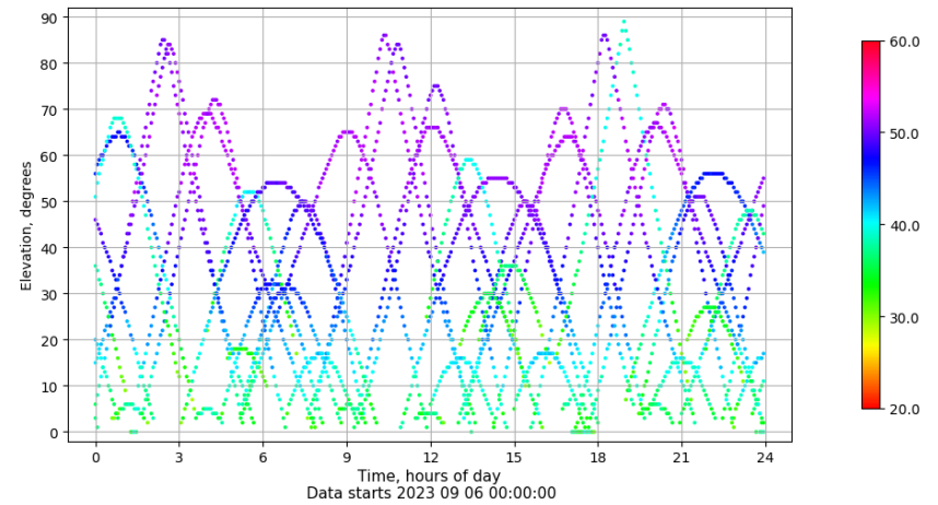
Time-elevation plot for station BADI. Signal to Noise S1C Data file BADI00ESP_R_2023249.xtr
