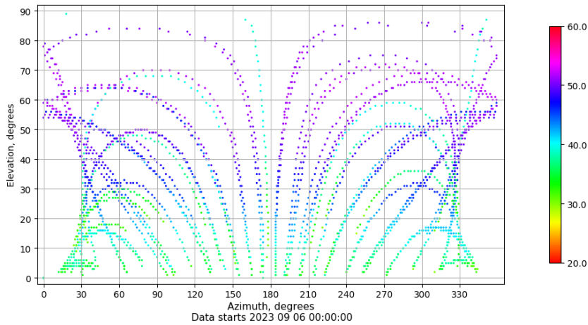
Azimuth-elevation plot for station BADI. Signal to Noise S1C Data file BADI00ESP_R_2023249.xtr
