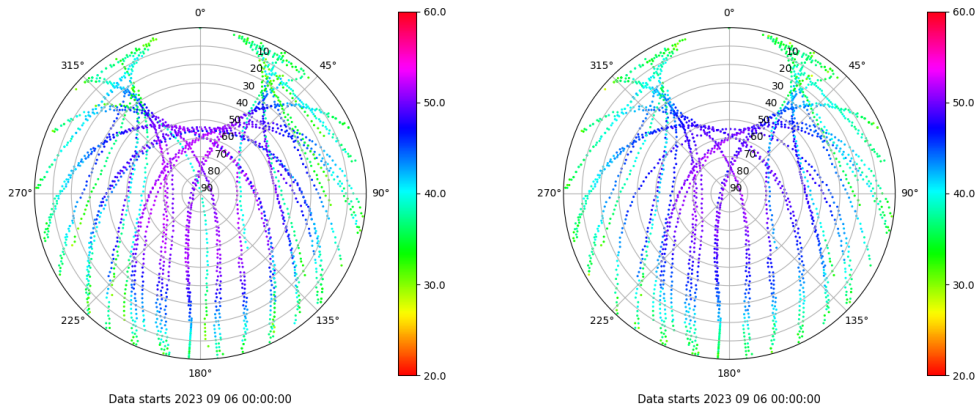
Skyplot for station BADI. Signal to Noise S1C Data file BADI00ESP_R_2023249.xtr Skyplot for station BADI. Signal to Noise S2C Data file BADI00ESP_R_2023249.xtr
