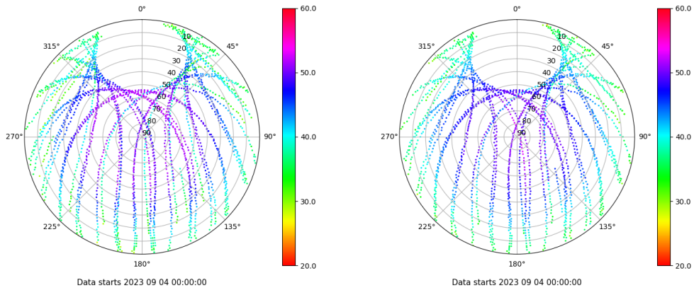
Skyplot for station BADI. Signal to Noise S1C Data file BADI00ESP_R_2023247.xtr Skyplot for station BADI. Signal to Noise S2C Data file BADI00ESP_R_2023247.xtr
