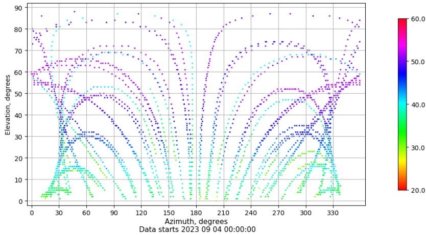
Azimuth-elevation plot for station BADI. Signal to Noise S1C Data file BADI00ESP_R_2023247.xtr
