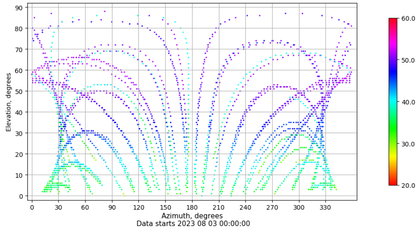
Azimuth-elevation plot for station BADI. Signal to Noise S1C Data file BADI00ESP_R_2023215.xtr
