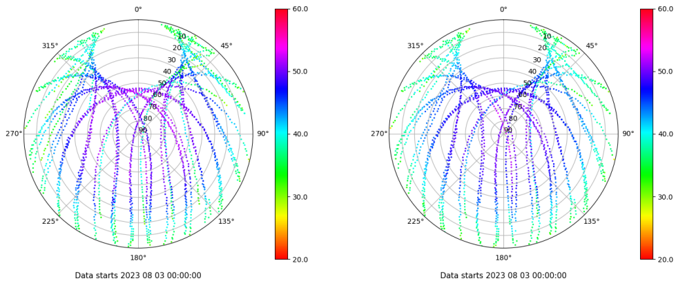
Skyplot for station BADI. Signal to Noise S1C Data file BADI00ESP_R_2023215.xtr Skyplot for station BADI. Signal to Noise S2C Data file BADI00ESP_R_2023215.xtr
