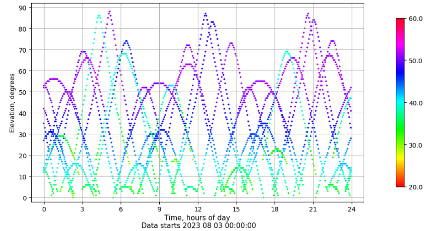
Time-elevation plot for station BADI. Signal to Noise S1C Data file BADI00ESP_R_2023215.xtr
