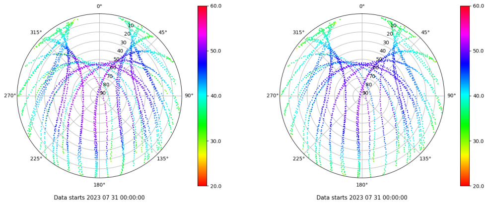
Skyplot for station BADI. Signal to Noise S1C Data file BADI00ESP_R_2023212.xtr Skyplot for station BADI. Signal to Noise S2C Data file BADI00ESP_R_2023212.xtr
