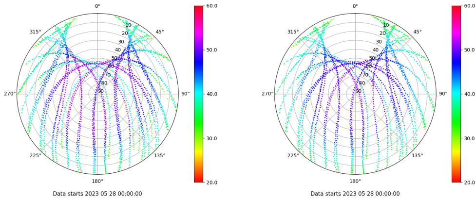
Skyplot for station BADI. Signal to Noise S1C Data file BADI00ESP_R_2023148.xtr Skyplot for station BADI. Signal to Noise S2C Data file BADI00ESP_R_2023148.xtr
