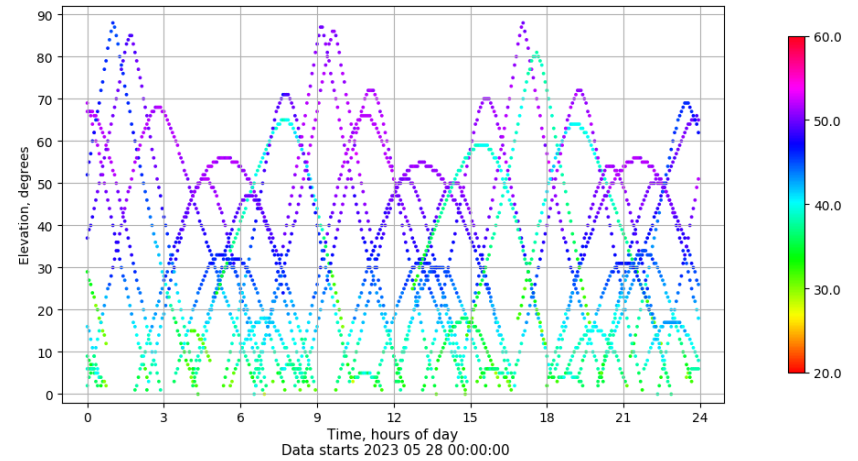
Time-elevation plot for station BADI. Signal to Noise S1C Data file BADI00ESP_R_2023148.xtr
