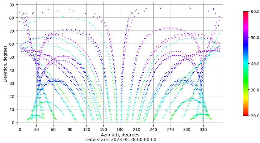
Azimuth-elevation plot for station BADI. Signal to Noise S1C Data file BADI00ESP_R_2023148.xtr
