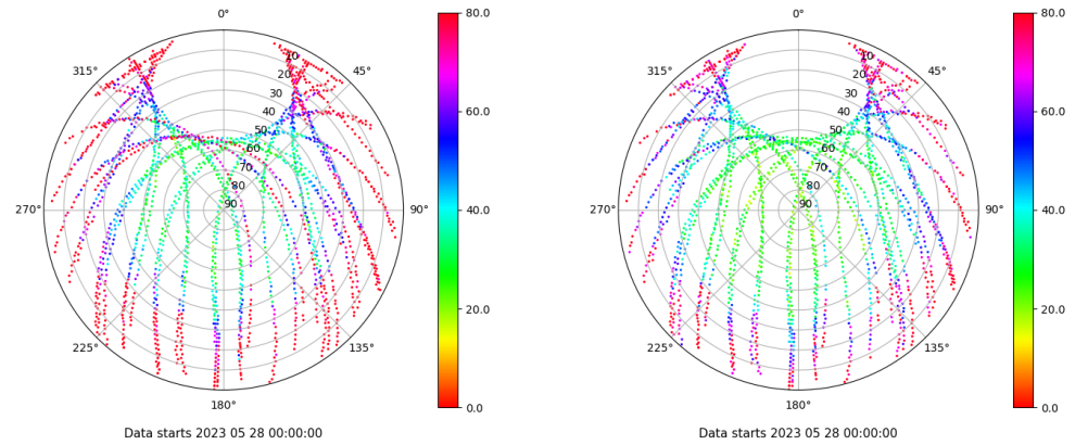
Skyplot for station BADI. Parameter M1C Data file BADI00ESP_R_2023148.xtr Skyplot for station BADI. Parameter M2C Data file BADI00ESP_R_2023148.xtr
