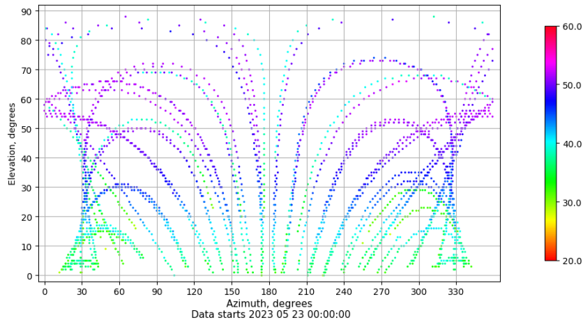
Azimuth-elevation plot for station BADI. Signal to Noise S1C Data file BADI00ESP_R_2023143.xtr
