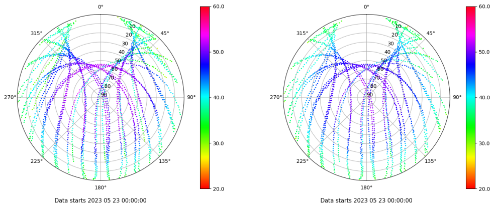
Skyplot for station BADI. Signal to Noise S1C Data file BADI00ESP_R_2023143.xtr Skyplot for station BADI. Signal to Noise S2C Data file BADI00ESP_R_2023143.xtr
