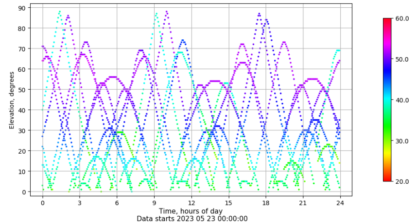
Time-elevation plot for station BADI. Signal to Noise S1C Data file BADI00ESP_R_2023143.xtr
