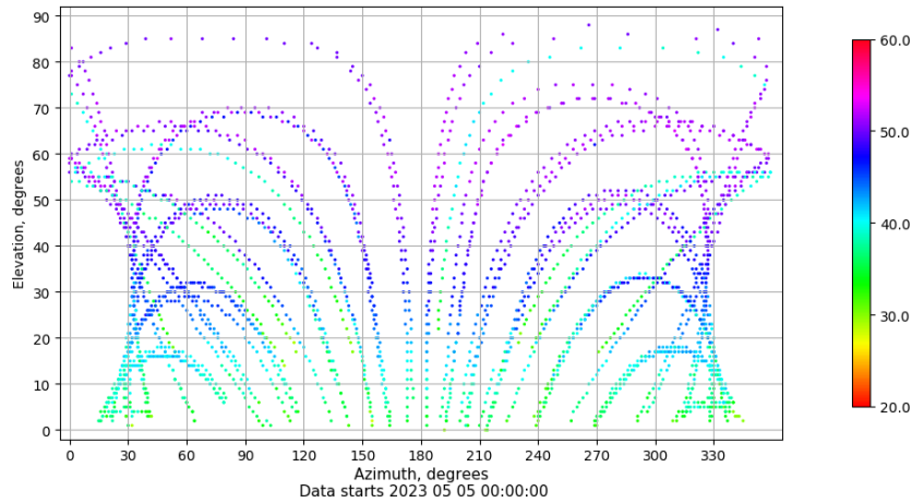
Azimuth-elevation plot for station BADI. Signal to Noise S1C Data file BADI00ESP_R_2023125.xtr
