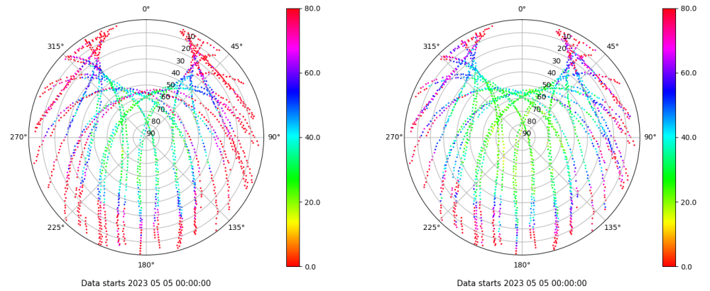
Skyplot for station BADI. Parameter M1C Data file BADI00ESP_R_2023125.xtr Skyplot for station BADI. Parameter M2C Data file BADI00ESP_R_2023125.xtr
