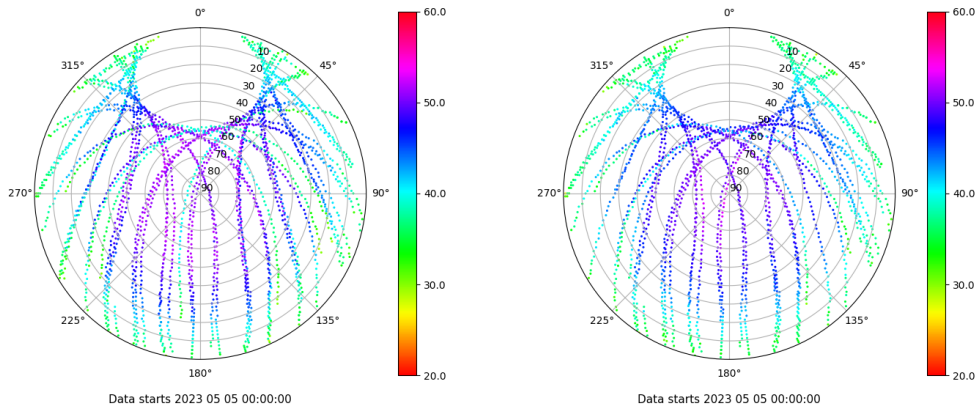
Skyplot for station BADI. Signal to Noise S1C Data file BADI00ESP_R_2023125.xtr Skyplot for station BADI. Signal to Noise S2C Data file BADI00ESP_R_2023125.xtr
