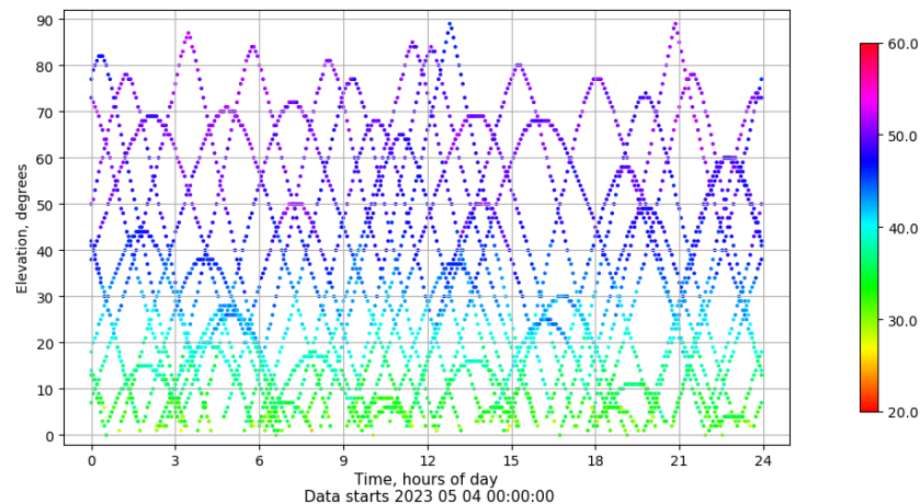
Time-elevation plot for station BADI. Signal to Noise S1C Data file BADI00ESP_R_2023124.xtr
