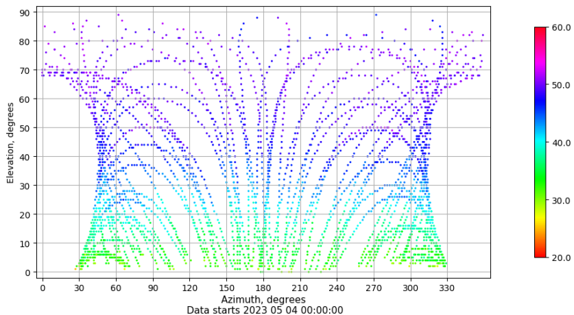
Azimuth-elevation plot for station BADI. Signal to Noise S1C Data file BADI00ESP_R_2023124.xtr
