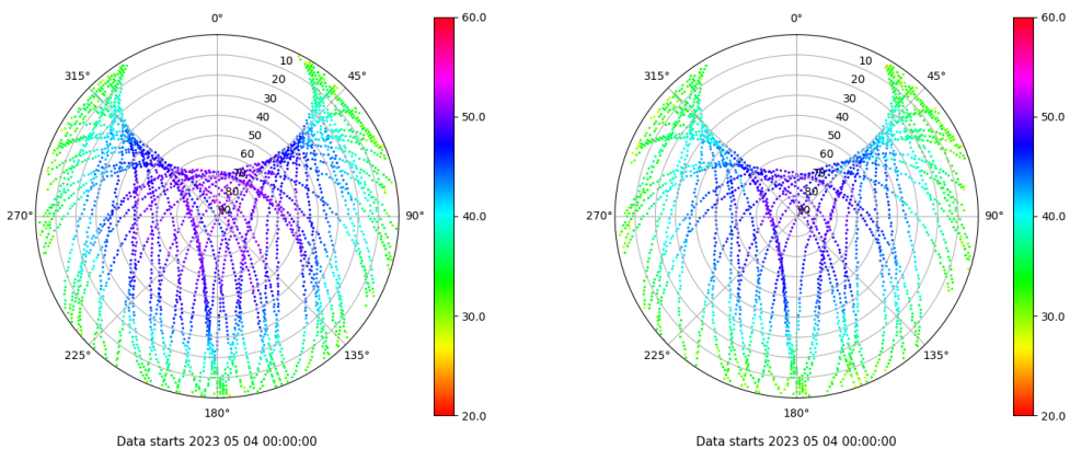
Skyplot for station BADI. Signal to Noise S1C Data file BADI00ESP_R_2023124.xtr Skyplot for station BADI. Signal to Noise S2L Data file BADI00ESP_R_2023124.xtr
