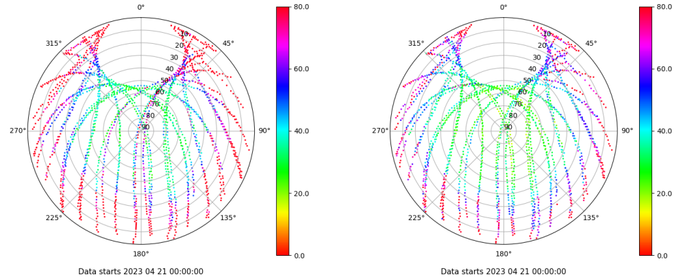
Skyplot for station BADI. Parameter M1C Data file BADI00ESP_R_2023111.xtr Skyplot for station BADI. Parameter M2C Data file BADI00ESP_R_2023111.xtr
