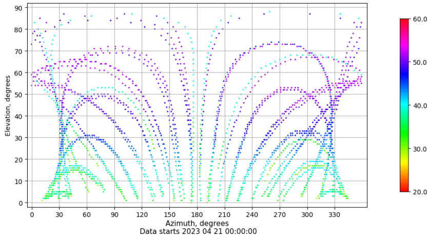
Azimuth-elevation plot for station BADI. Signal to Noise S1C Data file BADI00ESP_R_2023111.xtr
