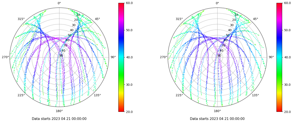
Skyplot for station BADI. Signal to Noise S1C Data file BADI00ESP_R_2023111.xtr Skyplot for station BADI. Signal to Noise S2C Data file BADI00ESP_R_2023111.xtr
