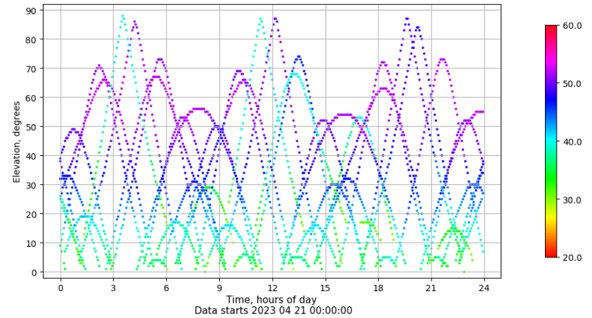
Time-elevation plot for station BADI. Signal to Noise S1C Data file BADI00ESP_R_2023111.xtr
