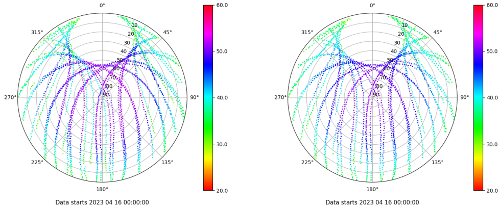
Skyplot for station BADI. Signal to Noise S1C Data file BADI00ESP_R_2023106.xtr Skyplot for station BADI. Signal to Noise S2C Data file BADI00ESP_R_2023106.xtr
