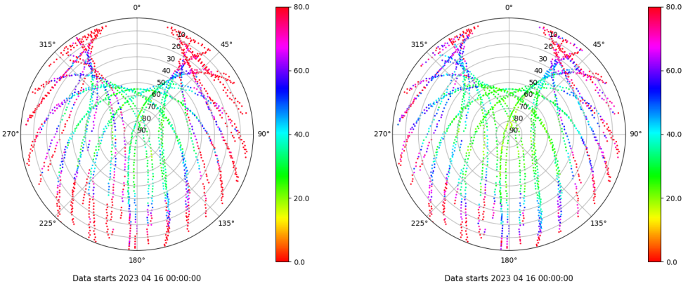
Skyplot for station BADI. Parameter M1C Data file BADI00ESP_R_2023106.xtr Skyplot for station BADI. Parameter M2C Data file BADI00ESP_R_2023106.xtr
