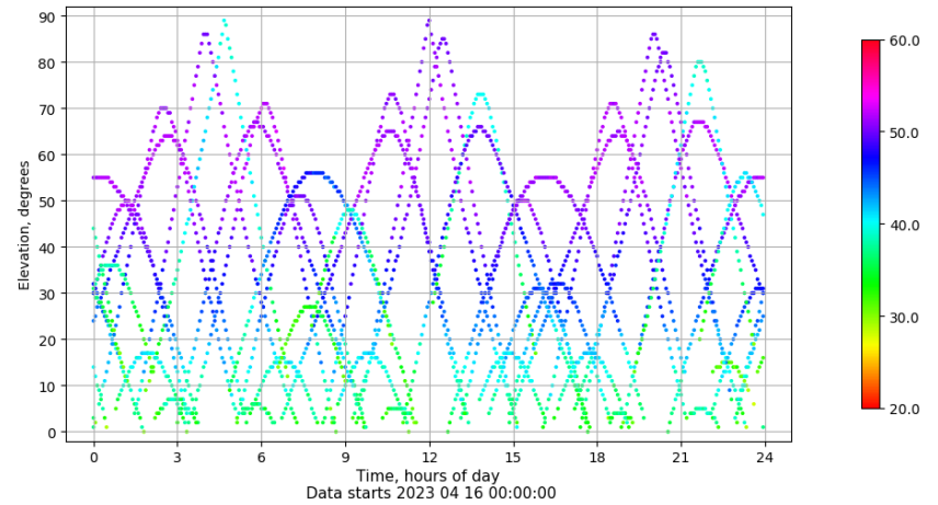
Time-elevation plot for station BADI. Signal to Noise S1C Data file BADI00ESP_R_2023106.xtr
