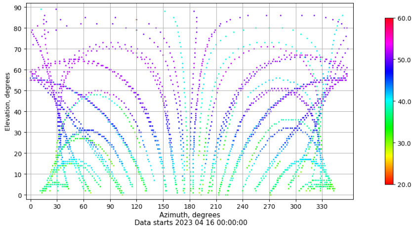
Azimuth-elevation plot for station BADI. Signal to Noise S1C Data file BADI00ESP_R_2023106.xtr
