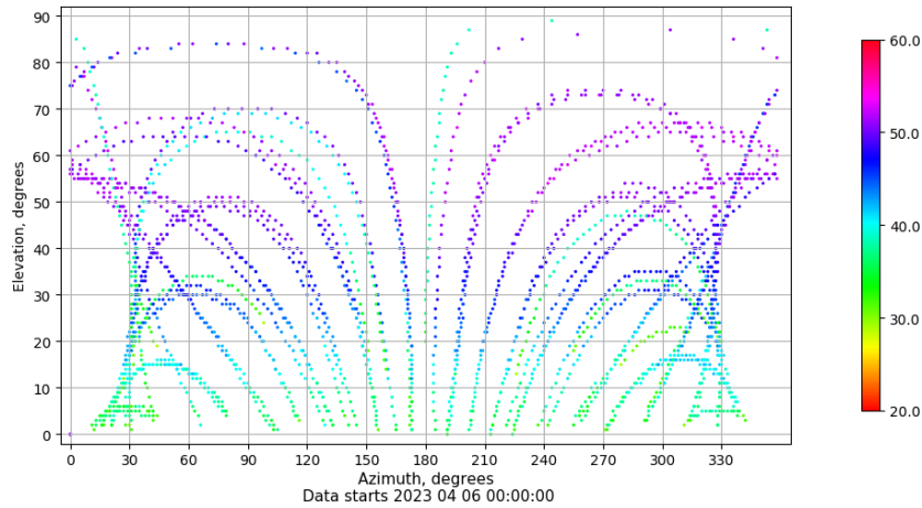
Azimuth-elevation plot for station BADI. Signal to Noise S1C Data file BADI00ESP_R_2023096.xtr
