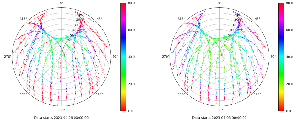
Skyplot for station BADI. Parameter M1C Data file BADI00ESP_R_2023096.xtr Skyplot for station BADI. Parameter M2C Data file BADI00ESP_R_2023096.xtr
