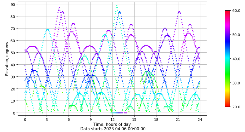
Time-elevation plot for station BADI. Signal to Noise S1C Data file BADI00ESP_R_2023096.xtr
