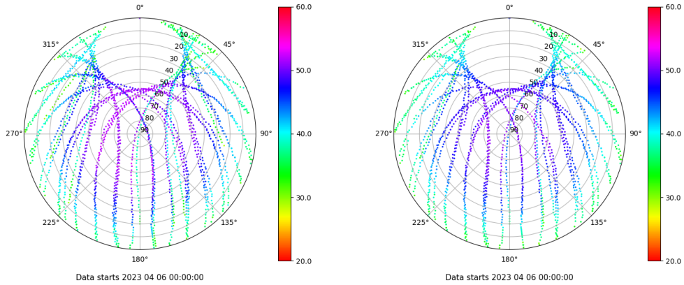
Skyplot for station BADI. Signal to Noise S1C Data file BADI00ESP_R_2023096.xtr Skyplot for station BADI. Signal to Noise S2C Data file BADI00ESP_R_2023096.xtr
