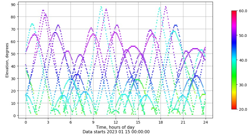
Time-elevation plot for station BADI. Signal to Noise S1C Data file BADI00ESP_R_2023015.xtr
