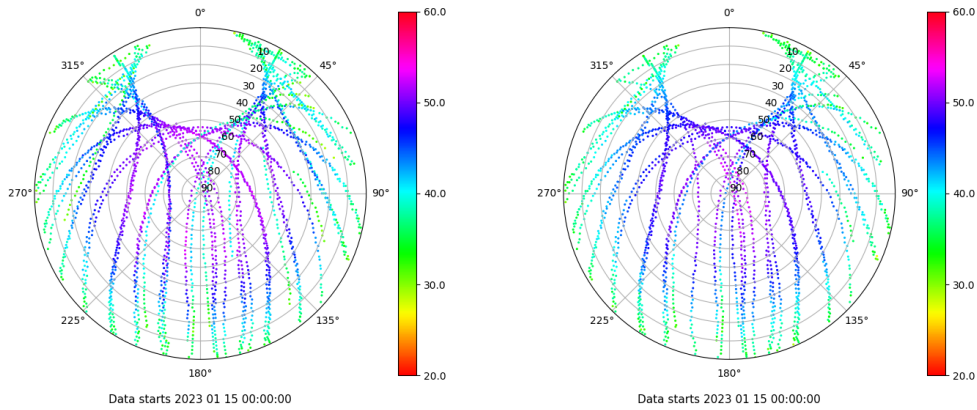
Skyplot for station BADI. Signal to Noise S1C Data file BADI00ESP_R_2023015.xtr Skyplot for station BADI. Signal to Noise S2C Data file BADI00ESP_R_2023015.xtr
