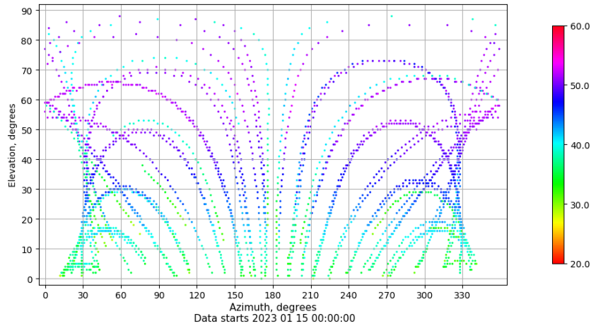
Azimuth-elevation plot for station BADI. Signal to Noise S1C Data file BADI00ESP_R_2023015.xtr
