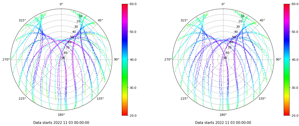
Skyplot for station BADI. Signal to Noise S1C Data file BADI00ESP_R_2022307.xtr Skyplot for station BADI. Signal to Noise S2C Data file BADI00ESP_R_2022307.xtr
