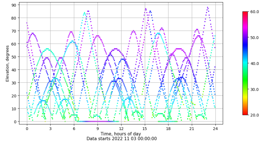
Time-elevation plot for station BADI. Signal to Noise S1C Data file BADI00ESP_R_2022307.xtr
