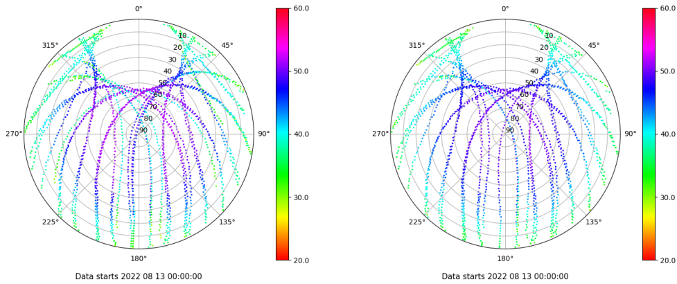
Skyplot for station BADI. Signal to Noise S1C Data file BADI00ESP_R_2022225.xtr Skyplot for station BADI. Signal to Noise S2C Data file BADI00ESP_R_2022225.xtr
