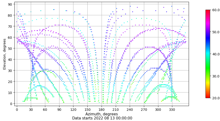
Azimuth-elevation plot for station BADI. Signal to Noise S1C Data file BADI00ESP_R_2022225.xtr
