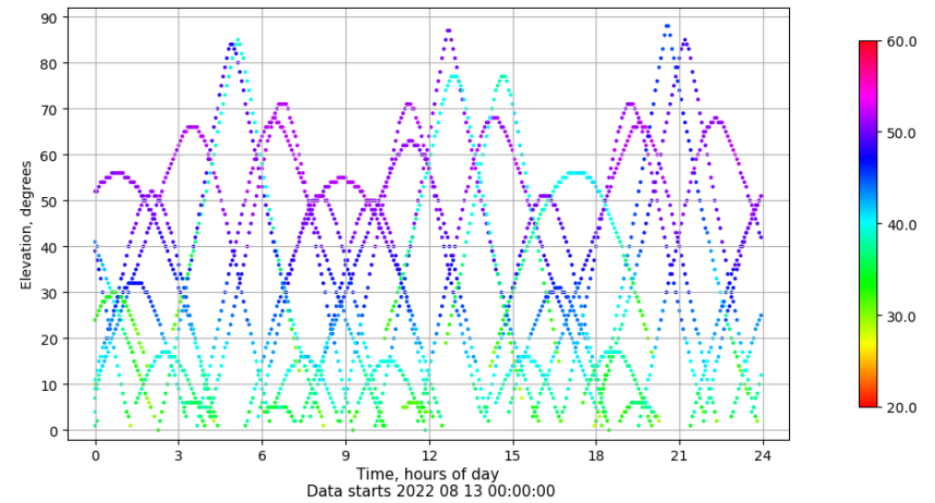
Time-elevation plot for station BADI. Signal to Noise S1C Data file BADI00ESP_R_2022225.xtr
