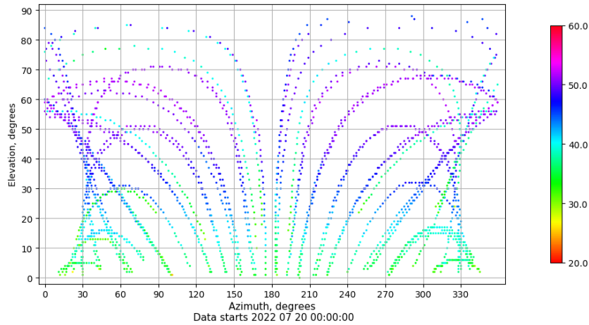
Azimuth-elevation plot for station BADI. Signal to Noise S1C Data file BADI00ESP_R_2022201.xtr
