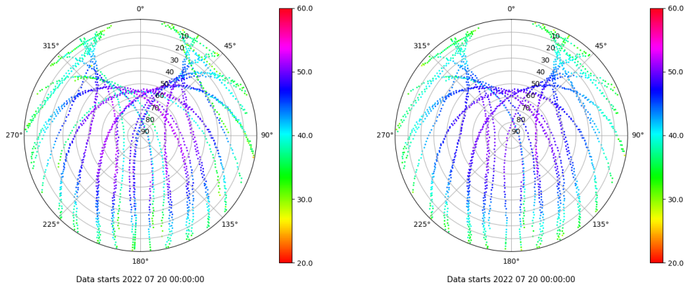
Skyplot for station BADI. Signal to Noise S1C Data file BADI00ESP_R_2022201.xtr Skyplot for station BADI. Signal to Noise S2C Data file BADI00ESP_R_2022201.xtr
