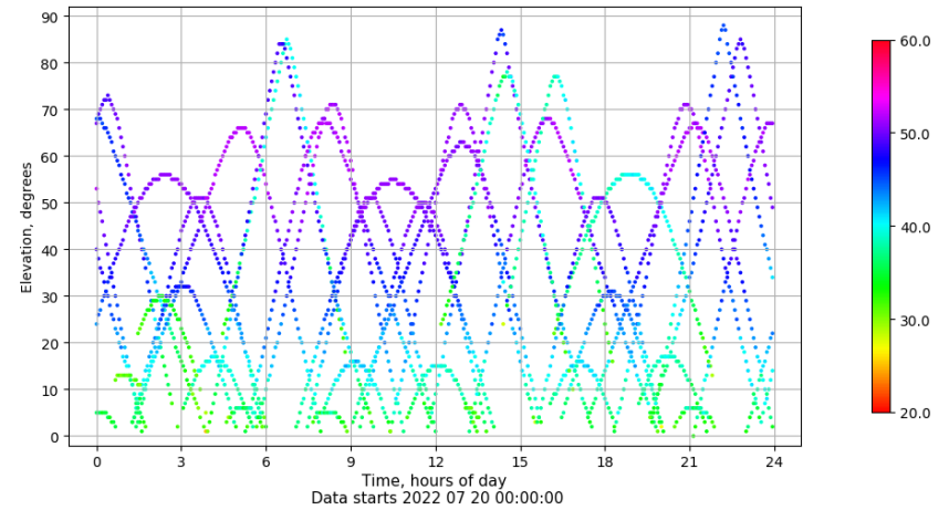
Time-elevation plot for station BADI. Signal to Noise S1C Data file BADI00ESP_R_2022201.xtr
