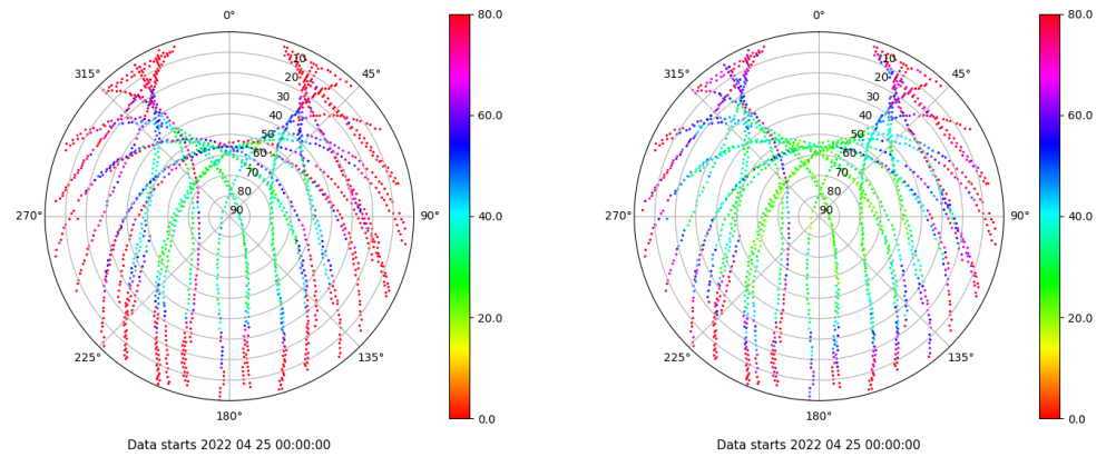
Skyplot for station BADI. Parameter M1C Data file BADI00ESP_R_2022115.xtr Skyplot for station BADI. Parameter M2C Data file BADI00ESP_R_2022115.xtr
