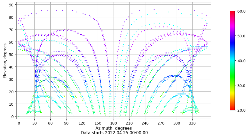
Azimuth-elevation plot for station BADI. Signal to Noise S1C Data file BADI00ESP_R_2022115.xtr
