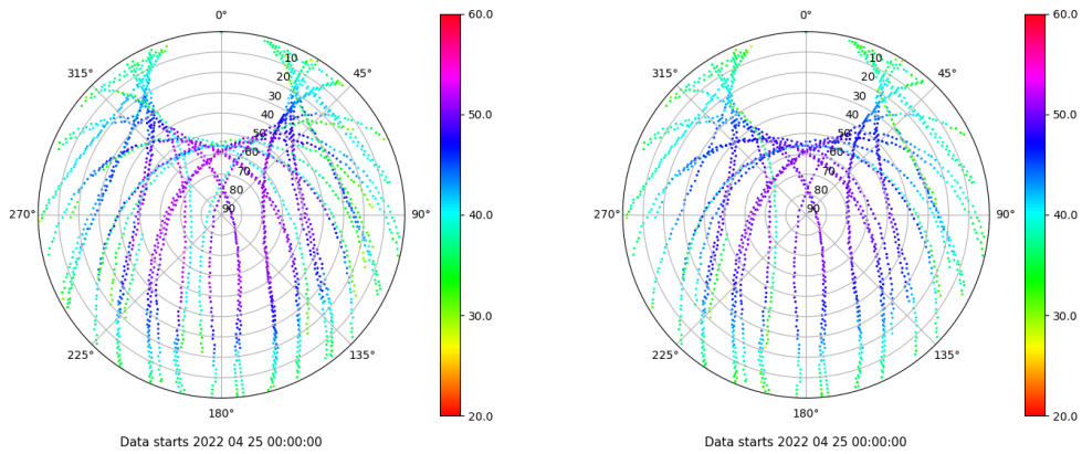
Skyplot for station BADI. Signal to Noise S1C Data file BADI00ESP_R_2022115.xtr Skyplot for station BADI. Signal to Noise S2C Data file BADI00ESP_R_2022115.xtr
