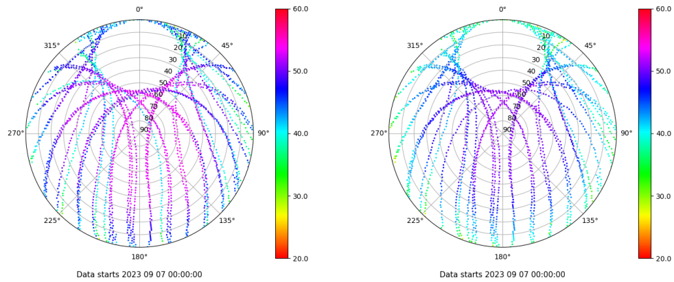
Skyplot for station ALOR. Signal to Noise S1C Data file ALOR00ESP_R_2023250.xtr Skyplot for station ALOR. Signal to Noise S2P Data file ALOR00ESP_R_2023250.xtr
