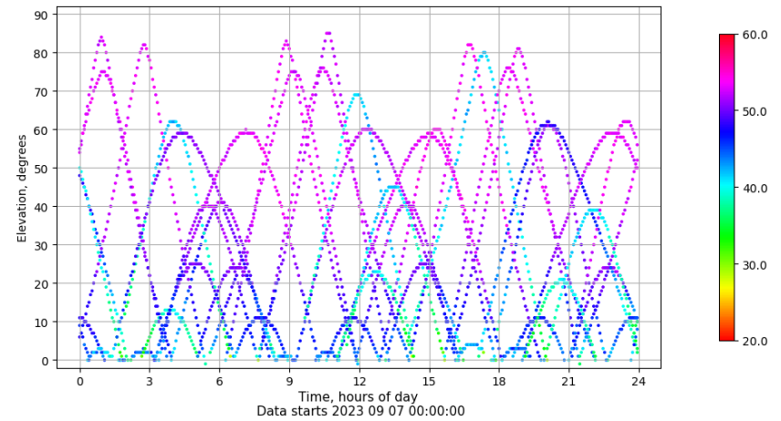
Time-elevation plot for station ALOR. Signal to Noise S1C Data file ALOR00ESP_R_2023250.xtr
