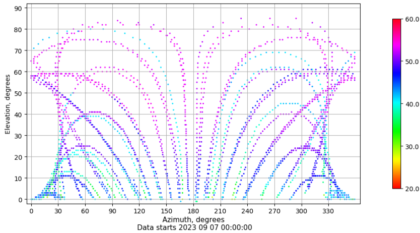
Azimuth-elevation plot for station ALOR. Signal to Noise S1C Data file ALOR00ESP_R_2023250.xtr
