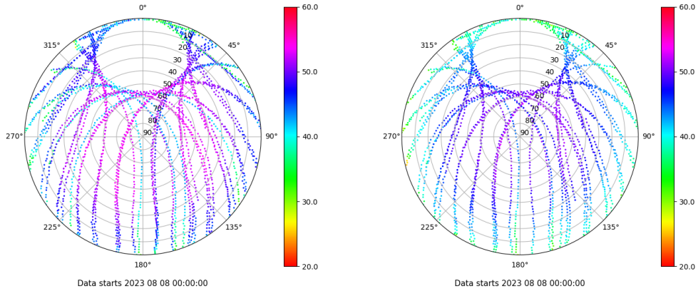
Skyplot for station ALOR. Signal to Noise S1C Data file ALOR00ESP_R_2023220.xtr Skyplot for station ALOR. Signal to Noise S2P Data file ALOR00ESP_R_2023220.xtr
