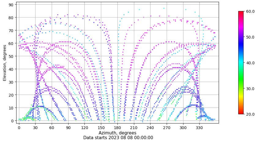
Azimuth-elevation plot for station ALOR. Signal to Noise S1C Data file ALOR00ESP_R_2023220.xtr
