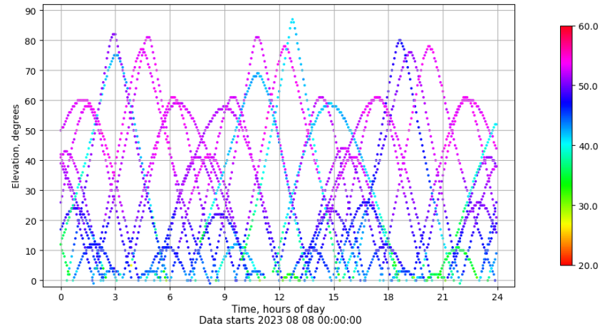
Time-elevation plot for station ALOR. Signal to Noise S1C Data file ALOR00ESP_R_2023220.xtr
