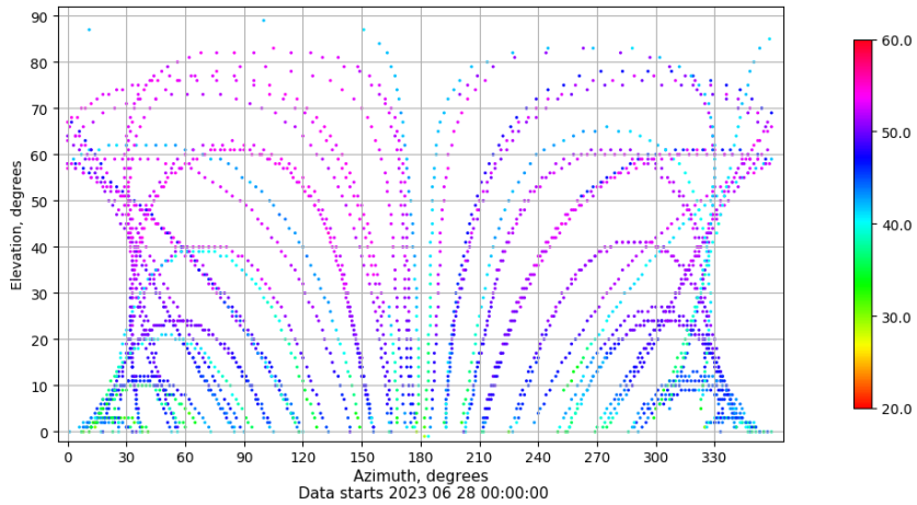
Azimuth-elevation plot for station ALOR. Signal to Noise S1C Data file ALOR00ESP_R_2023179.xtr
