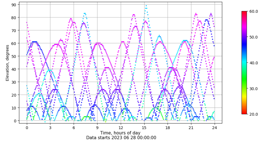
Time-elevation plot for station ALOR. Signal to Noise S1C Data file ALOR00ESP_R_2023179.xtr
