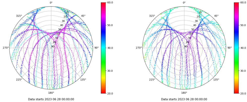
Skyplot for station ALOR. Signal to Noise S1C Data file ALOR00ESP_R_2023179.xtr Skyplot for station ALOR. Signal to Noise S2P Data file ALOR00ESP_R_2023179.xtr
