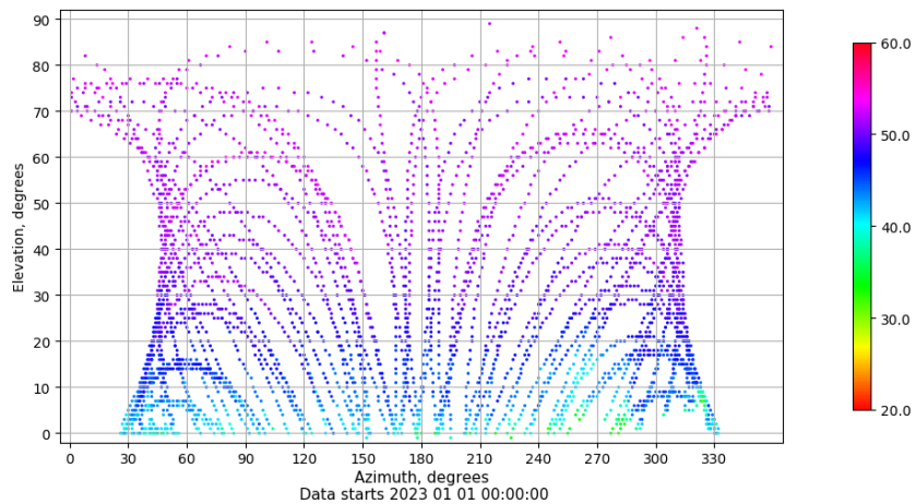
Azimuth-elevation plot for station ALOR. Signal to Noise S1C Data file ALOR00ESP_R_2023001.xtr
