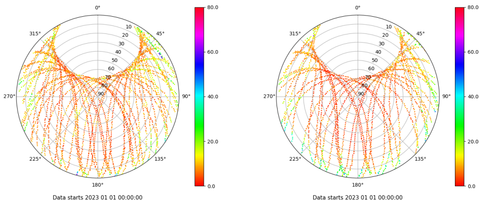
Skyplot for station ALOR. Parameter M1C Data file ALOR00ESP_R_2023001.xtr Skyplot for station ALOR. Parameter M2S Data file ALOR00ESP_R_2023001.xtr
