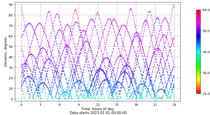
Time-elevation plot for station ALOR. Signal to Noise S1C Data file ALOR00ESP_R_2023001.xtr
