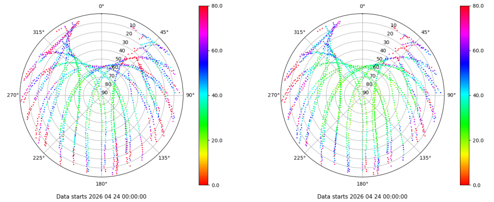
Skyplot for station ALC1. Parameter M1C Data file ALC100ESP_R_2026114.xtr Skyplot for station ALC1. Parameter M2C Data file ALC100ESP_R_2026114.xtr
