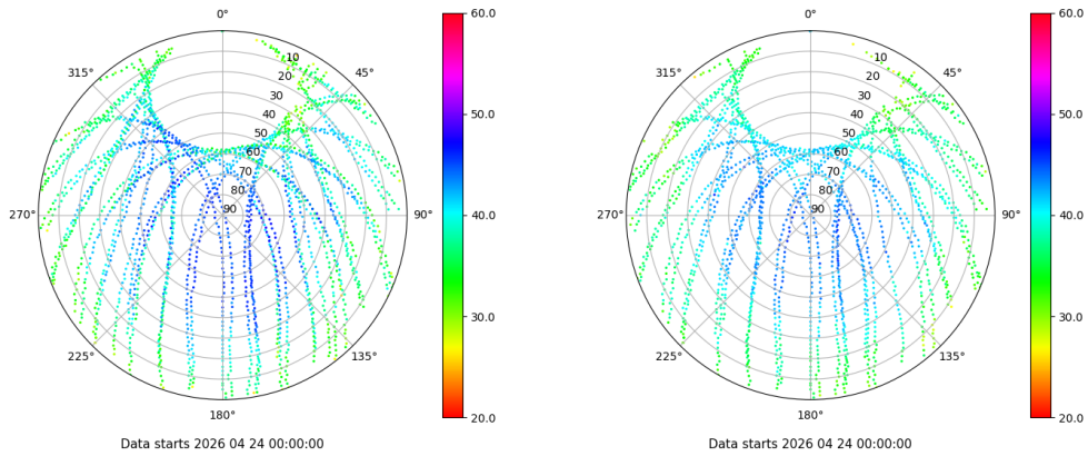
Skyplot for station ALC1. Signal to Noise S1C Data file ALC100ESP_R_2026114.xtr Skyplot for station ALC1. Signal to Noise S2C Data file ALC100ESP_R_2026114.xtr
