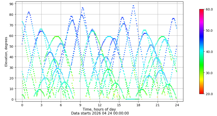
Time-elevation plot for station ALC1. Signal to Noise S1C Data file ALC100ESP_R_2026114.xtr
