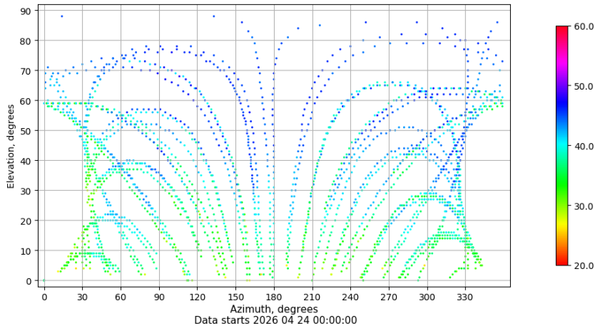
Azimuth-elevation plot for station ALC1. Signal to Noise S1C Data file ALC100ESP_R_2026114.xtr
