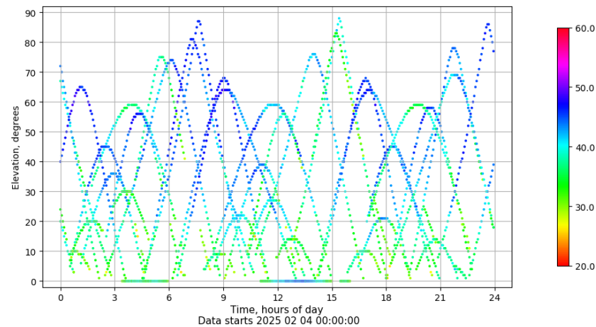
Time-elevation plot for station ALC1. Signal to Noise S1C Data file ALC100ESP_R_2025035.xtr
