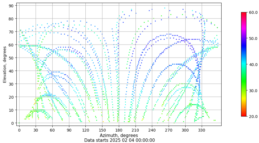
Azimuth-elevation plot for station ALC1. Signal to Noise S1C Data file ALC100ESP_R_2025035.xtr
