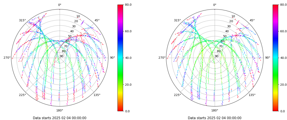
Skyplot for station ALC1. Parameter M1C Data file ALC100ESP_R_2025035.xtr Skyplot for station ALC1. Parameter M2C Data file ALC100ESP_R_2025035.xtr
