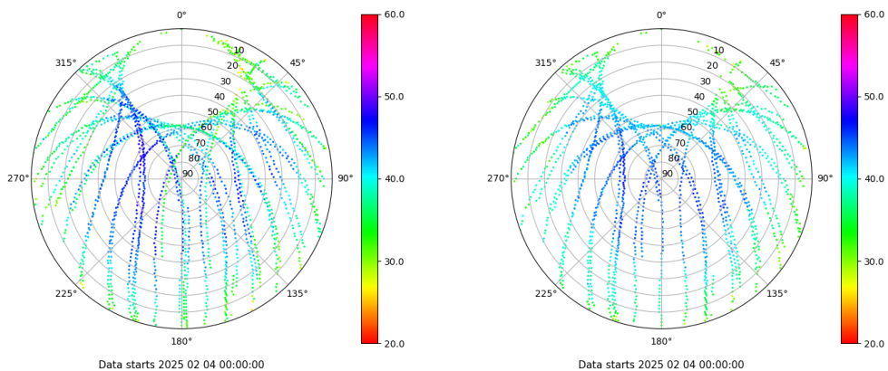
Skyplot for station ALC1. Signal to Noise S1C Data file ALC100ESP_R_2025035.xtr Skyplot for station ALC1. Signal to Noise S2C Data file ALC100ESP_R_2025035.xtr
