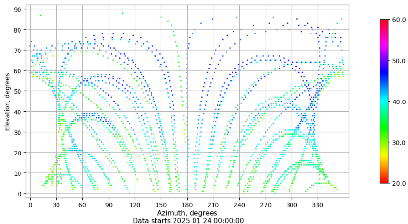
Azimuth-elevation plot for station ALC1. Signal to Noise S1C Data file ALC100ESP_R_2025024.xtr
