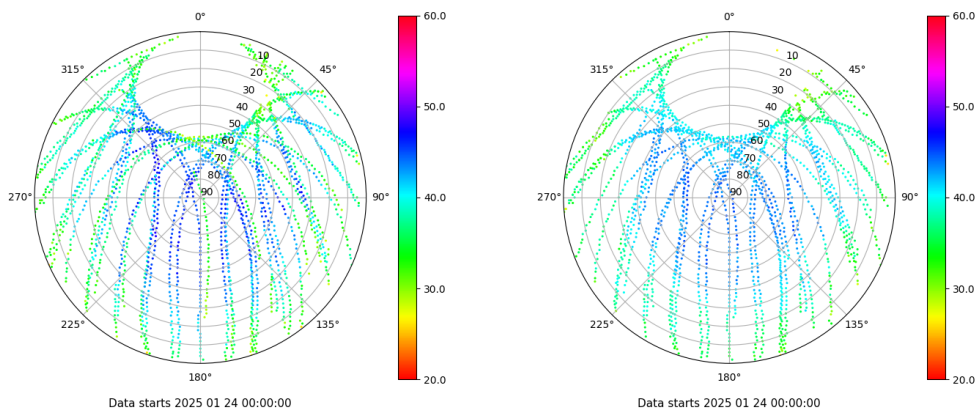
Skyplot for station ALC1. Signal to Noise S1C Data file ALC100ESP_R_2025024.xtr Skyplot for station ALC1. Signal to Noise S2C Data file ALC100ESP_R_2025024.xtr
