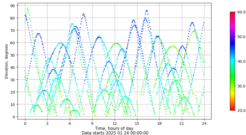
Time-elevation plot for station ALC1. Signal to Noise S1C Data file ALC100ESP_R_2025024.xtr
