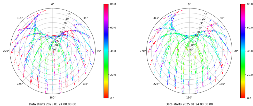
Skyplot for station ALC1. Parameter M1C Data file ALC100ESP_R_2025024.xtr Skyplot for station ALC1. Parameter M2C Data file ALC100ESP_R_2025024.xtr
