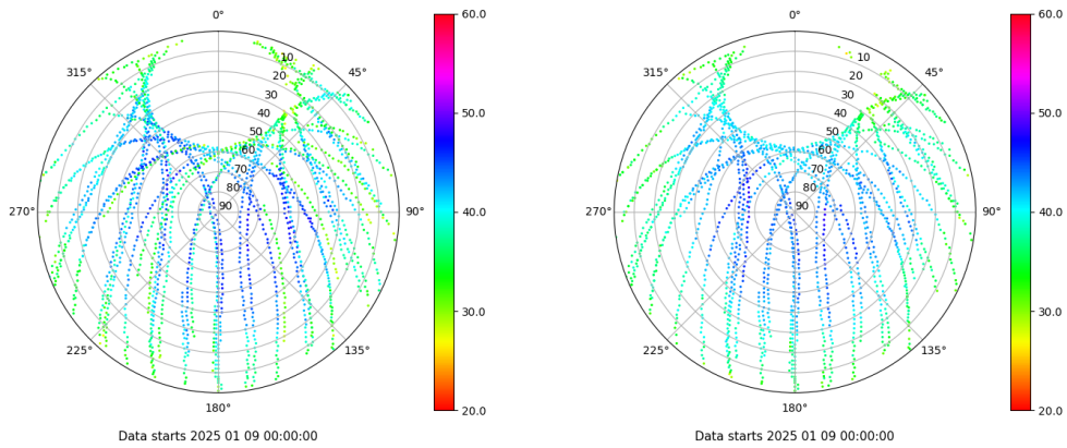
Skyplot for station ALC1. Signal to Noise S1C Data file ALC100ESP_R_2025009.xtr Skyplot for station ALC1. Signal to Noise S2C Data file ALC100ESP_R_2025009.xtr
