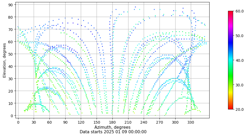
Azimuth-elevation plot for station ALC1. Signal to Noise S1C Data file ALC100ESP_R_2025009.xtr
