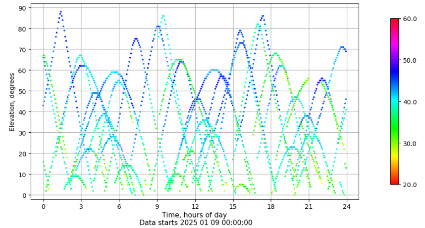
Time-elevation plot for station ALC1. Signal to Noise S1C Data file ALC100ESP_R_2025009.xtr
