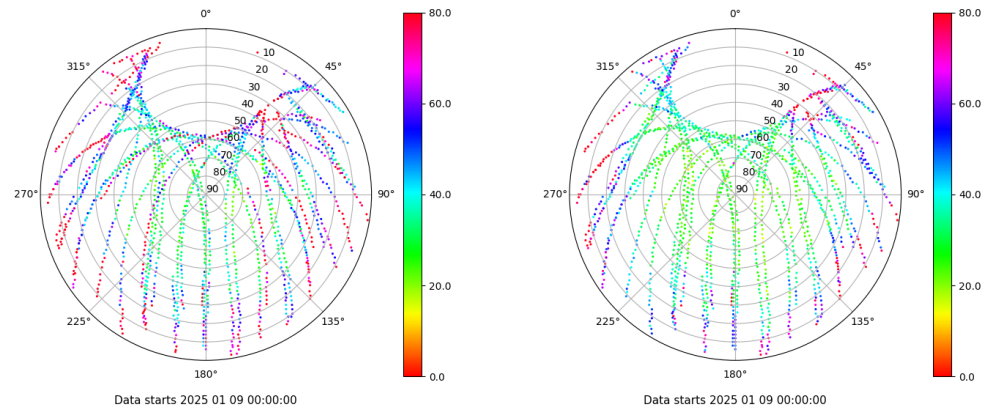
Skyplot for station ALC1. Parameter M1C Data file ALC100ESP_R_2025009.xtr Skyplot for station ALC1. Parameter M2C Data file ALC100ESP_R_2025009.xtr
