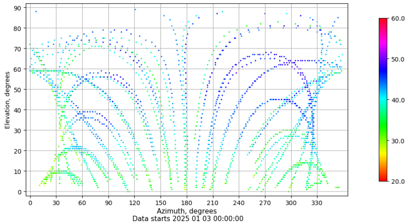
Azimuth-elevation plot for station ALC1. Signal to Noise S1C Data file ALC100ESP_R_2025003.xtr
