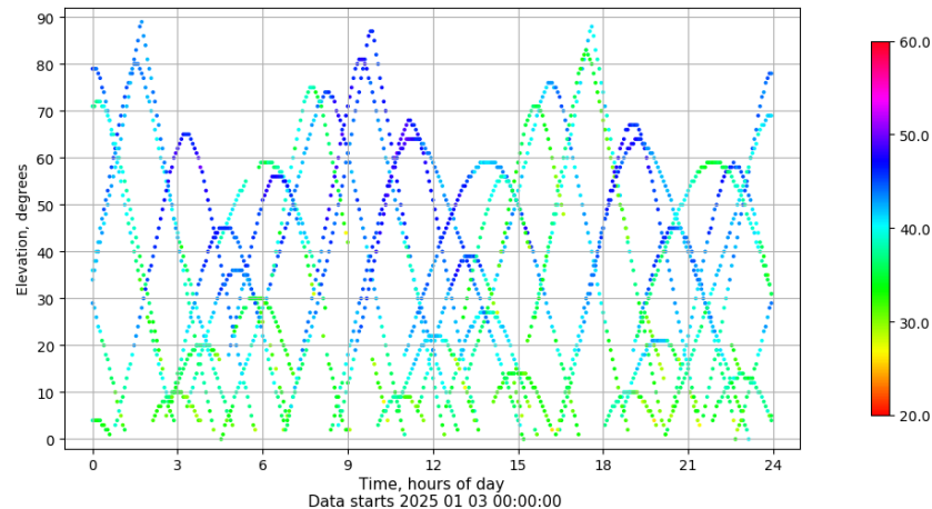
Time-elevation plot for station ALC1. Signal to Noise S1C Data file ALC100ESP_R_2025003.xtr
