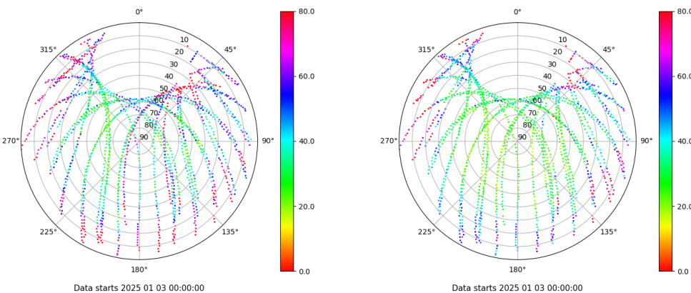
Skyplot for station ALC1. Parameter M1C Data file ALC100ESP_R_2025003.xtr Skyplot for station ALC1. Parameter M2C Data file ALC100ESP_R_2025003.xtr
