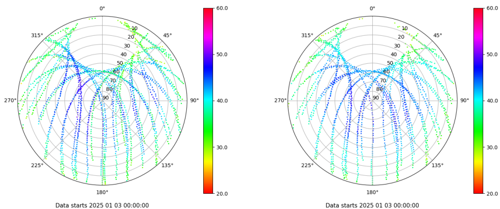
Skyplot for station ALC1. Signal to Noise S1C Data file ALC100ESP_R_2025003.xtr Skyplot for station ALC1. Signal to Noise S2C Data file ALC100ESP_R_2025003.xtr
