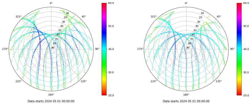
Skyplot for station ALC1. Signal to Noise S1C Data file ALC100ESP_R_2024122.xtr Skyplot for station ALC1. Signal to Noise S2C Data file ALC100ESP_R_2024122.xtr
