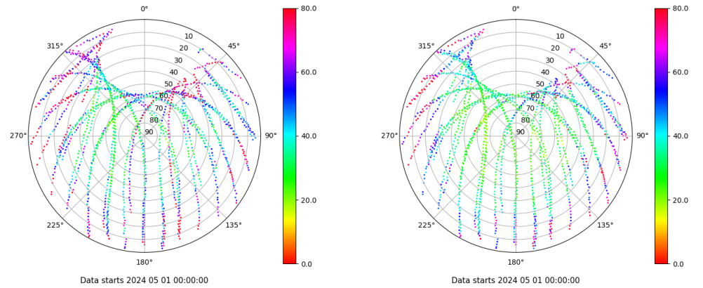
Skyplot for station ALC1. Parameter M1C Data file ALC100ESP_R_2024122.xtr Skyplot for station ALC1. Parameter M2C Data file ALC100ESP_R_2024122.xtr
