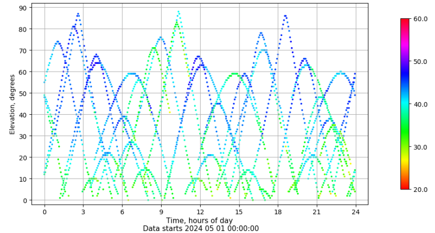
Time-elevation plot for station ALC1. Signal to Noise S1C Data file ALC100ESP_R_2024122.xtr
