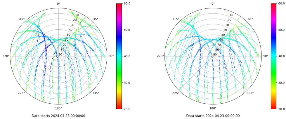
Skyplot for station ALC1. Signal to Noise S1C Data file ALC100ESP_R_2024114.xtr Skyplot for station ALC1. Signal to Noise S2C Data file ALC100ESP_R_2024114.xtr
