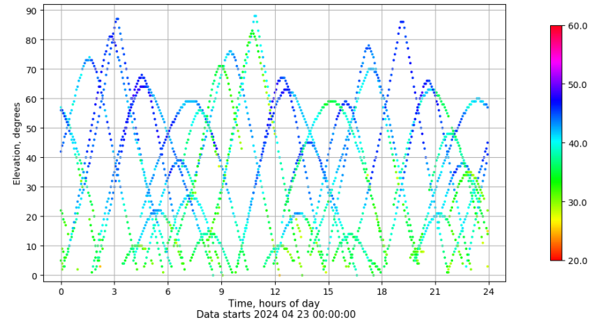
Time-elevation plot for station ALC1. Signal to Noise S1C Data file ALC100ESP_R_2024114.xtr
