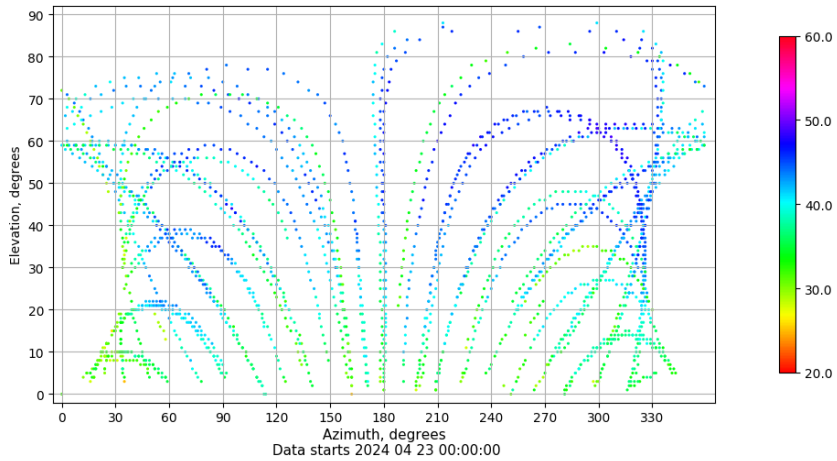
Azimuth-elevation plot for station ALC1. Signal to Noise S1C Data file ALC100ESP_R_2024114.xtr
