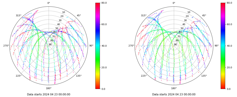
Skyplot for station ALC1. Parameter M1C Data file ALC100ESP_R_2024114.xtr Skyplot for station ALC1. Parameter M2C Data file ALC100ESP_R_2024114.xtr
