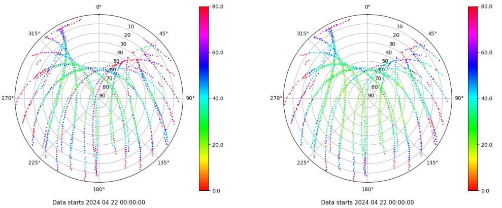
Skyplot for station ALC1. Parameter M1C Data file ALC100ESP_R_2024113.xtr Skyplot for station ALC1. Parameter M2C Data file ALC100ESP_R_2024113.xtr
