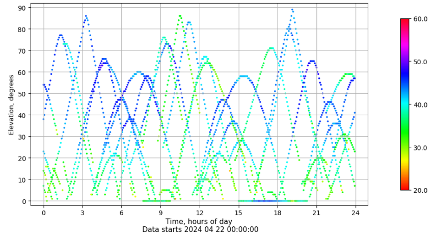
Time-elevation plot for station ALC1. Signal to Noise S1C Data file ALC100ESP_R_2024113.xtr
