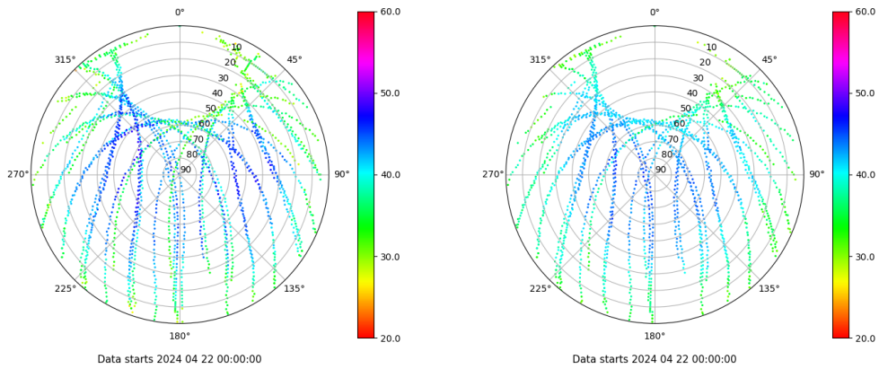
Skyplot for station ALC1. Signal to Noise S1C Data file ALC100ESP_R_2024113.xtr Skyplot for station ALC1. Signal to Noise S2C Data file ALC100ESP_R_2024113.xtr
