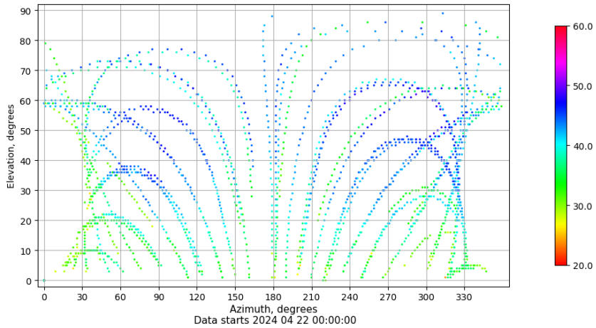
Azimuth-elevation plot for station ALC1. Signal to Noise S1C Data file ALC100ESP_R_2024113.xtr
