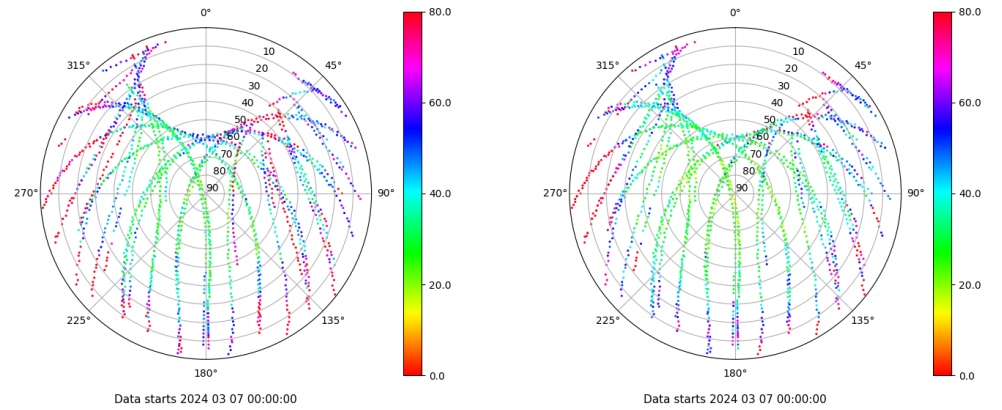
Skyplot for station ALC1. Parameter M1C Data file ALC100ESP_R_2024067.xtr Skyplot for station ALC1. Parameter M2C Data file ALC100ESP_R_2024067.xtr
