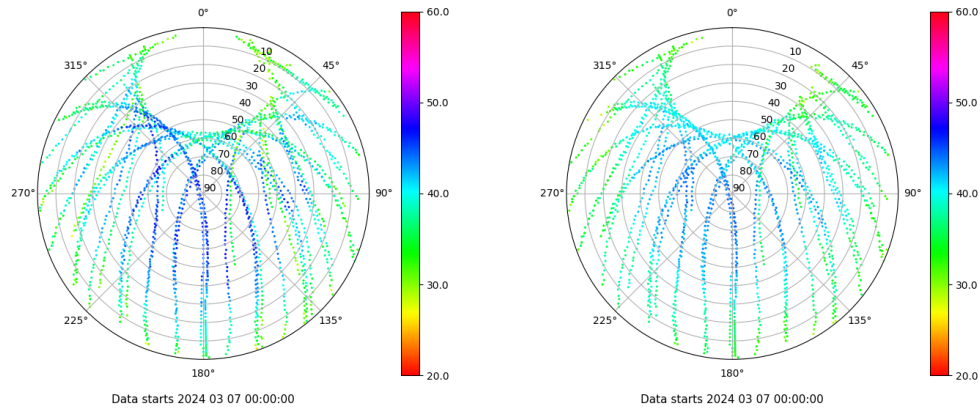
Skyplot for station ALC1. Signal to Noise S1C Data file ALC100ESP_R_2024067.xtr Skyplot for station ALC1. Signal to Noise S2C Data file ALC100ESP_R_2024067.xtr
