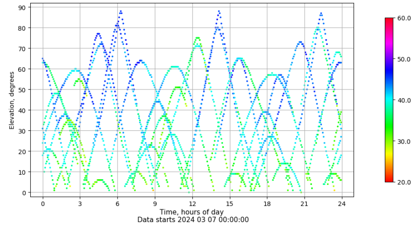
Time-elevation plot for station ALC1. Signal to Noise S1C Data file ALC100ESP_R_2024067.xtr
