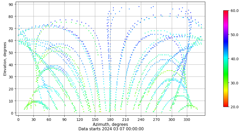
Azimuth-elevation plot for station ALC1. Signal to Noise S1C Data file ALC100ESP_R_2024067.xtr
